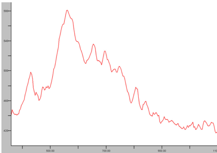
Fig. 3: CL spectral response corresponding to an area of \approx 2.5 \times 2 mm through a 50 nm-thick \text{Si}_3\text{N}_4 window. The conditions are 17 keV, 80 \mu A, Ar pressure of 40 \times 10^{-3} mbar and 0 mbar \text{CO}_2 pressure as used for Fig. 4 on Plate 1
