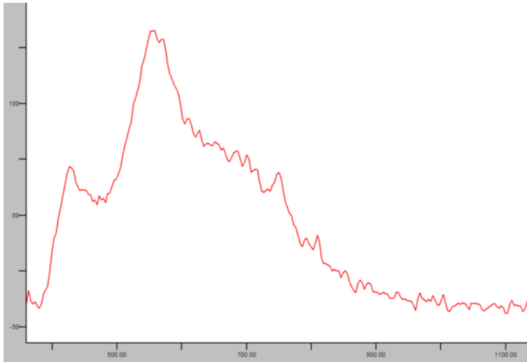
Fig. 2: CL spectral response corresponding to an area of \approx 2.5 \times 2 mm. The conditions are 17 keV, 80 \mu A, Ar pressure of < 40 \times 10^{-3} mbar and 0 mbar \text{CO}_2 pressure as used for Fig. 3 on Plate 1
