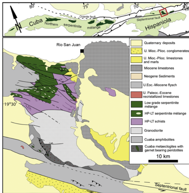
Figure 1. Geological map of Rio San Juan Complex (Dominican Republic, Hispaniola island), belonging to the Northern Serpentinite Mélange (modified after Draper and Nagle [1991]).
