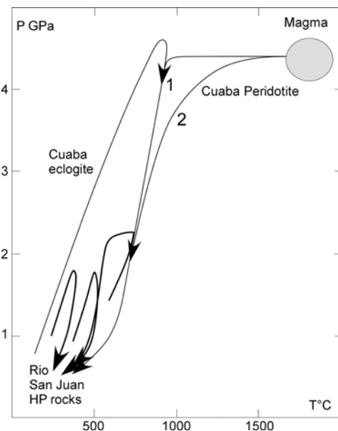
Figure 2. Proposed P-T paths for Cuaba garnet-bearing ultramafic rocks and associated eclogites (modified from Abbott et al. [2006]). Path 1: incorporation of the Cuaba peridotites into the oceanic eclogitic unit at UHP conditions. Path 2: incorporation of the Cuaba peridotites into the oceanic eclogitic unit at HP conditions. The P-T paths of the low pressure eclogites and associated blueschists (HP rocks) observed in the Northern Serpentinite Mélange are also reported (after Krebs et al. [2007]).
