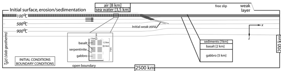
Figure 3. Two-dimensional numerical setting employed in this study showing initial distribution of different rock lithologies. The low-spreading oceanic crust (7 km thick) is composed by blocks of basalt and gabbro (1 km × 0.5 km) embedded in a serpentine matrix. The upper mantle is composed of dry peridotites. The upper plate is composed of a classical oceanic crust (sediment, basalt, and gabbro) above an initial dry peridotitic mantle. Initial temperature field (isotherms in °C) and boundary conditions are from Gorczyk et al. [2007]. Numerical grid steps: 2 km in the area of interest, 10 km outside area of interest. See text for detailed explanations.
