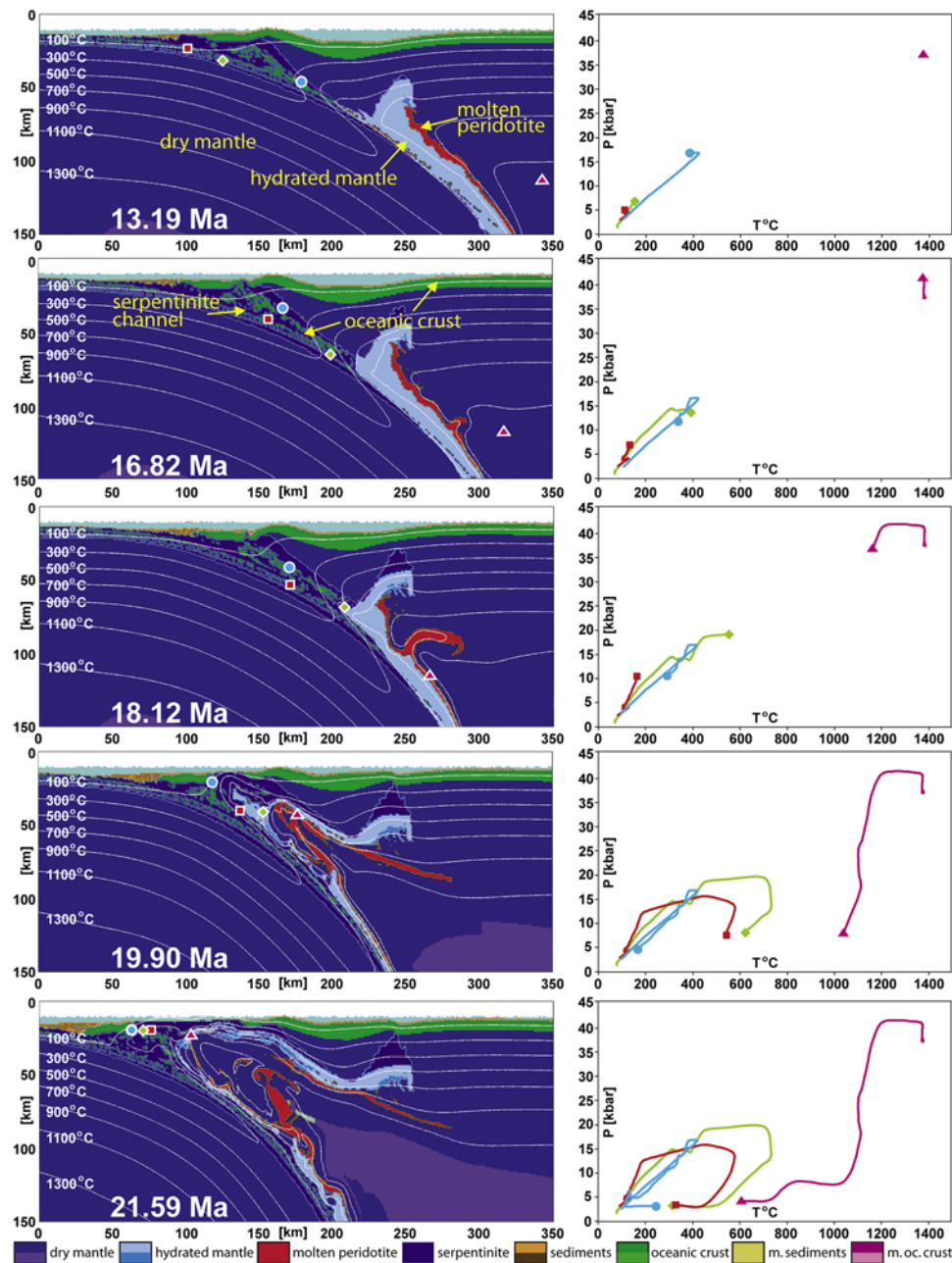
Figure 4. Final evolution of the 2-D model of the subduction of a slow spreading ridge in five time-step (total duration: 22 Ma). The colors of the geometrical shapes refer to the diagram with P-T paths and do not correspond to rock type. In the color code description “m.” stands for partially molten. The model reproduces the occurrence in the Rio San Juan complex of HP rocks in the front of the Northern Serpentine Mélange and garnet bearing peridotites at its rear. The model predicts that the exhumation of HP rocks occurred within the serpentinite channel coming from the subducted oceanic lithosphere. The garnet bearing peridotite derived from the mantle wedge and exhumed when the buoyant partially hydrated mantle (composed of partially dehydrated oceanic serpentinite and partially hydrated mantle wedge) is pushed toward the surface when the slab retreat and the asthenosphere upraise. Notice the occurrence of molten peridotite that could correspond to the observed Rio Boba intrusive (Figure 1).
