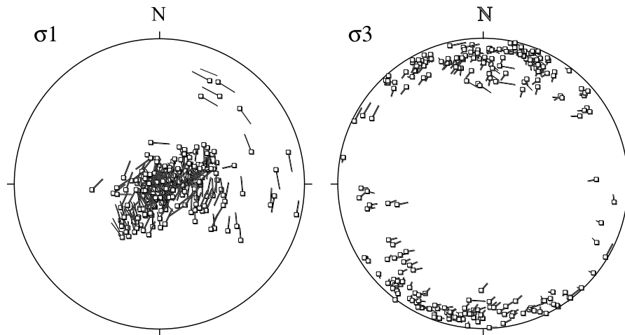
Figure 12. Dassu-Braldu area, results from the multiple inverse methods (software package mim5-miv4, A. Yamaji et al., Multiple Inverse Method Software Package, Freeware package, 2005, http://www.kueps.kyoto-u.ac.jp/~yamaji/PDS/indexe.html ); 235 points (from a 60 000 nodes grid) having a significant number of solutions tied to them [see Yamaji et al., 2005], plotted in lower hemisphere, equal-area projections. (left) Stereogram for \sigma_1 , clustered close to vertical. (right) Stereogram for \sigma_3 , with a poorly defined NNE-SSW best position.
