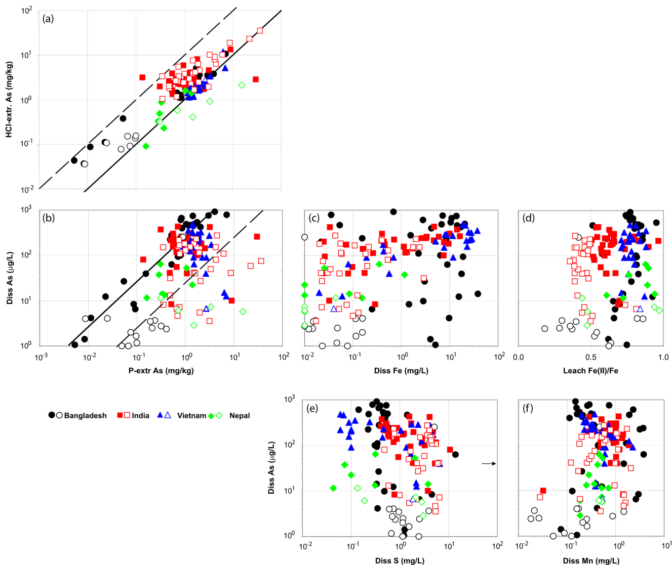
Fig. 2. Scatter plots of groundwater and aquifer particle properties for material collected with the needle-sampler in Bangladesh, India, Vietnam and Nepal. Note the logarithmic scale of all properties, with the exception of leachable Fe(II)/Fe ratios. Open symbols identify samples collected from insufficiently reducing samples, as identified in van Geen et al. (2008) by either leachable Fe(II)/Fe <0.5 or dissolved Fe concentrations <0.2 mg/L in samples with dissolved As <10 µg/L. Solid and dashed lines in (a) correspond to equal and 10-fold higher As concentrations in HCl-extractions, respectively, compared to As levels in P-extractions. Solid line and dashed lines in (b) correspond to K_d = 4 and 40 \text{ cm}^3/\text{g} , respectively. The arrow in (d) points to a single sample from Bangladesh containing an unexplained and extremely elevated level of 190 mg S/L.
