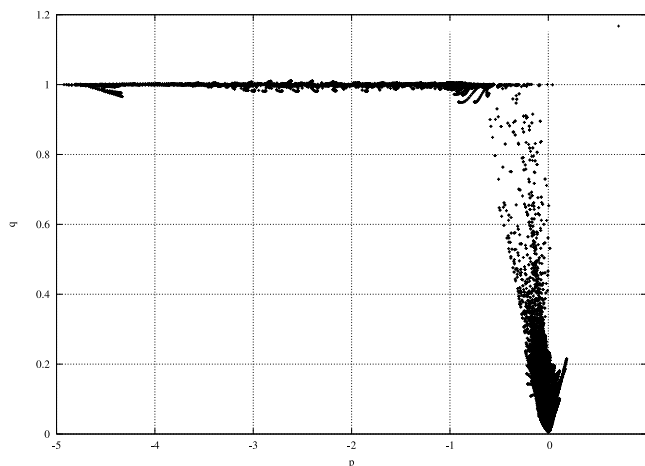
Figure 15. The qp -gram corresponding to the solution of the plane strain experiment. The quantity q = 2\mu'E_2' shows an upper bound which is the yield stress k = 1 of the material.
