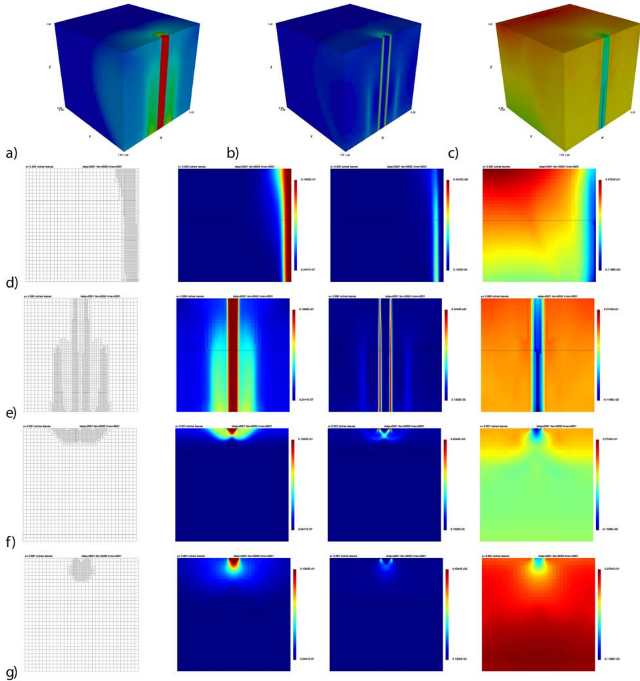
Figure 19. (a) Velocity norm field; (b) E_2' field; (c) pressure field; (d–g) cross sections of the grid, the velocity field, the E_2' field and the pressure field in planes x = 0.5, y = 1, z = 0 , and z = 1 .
