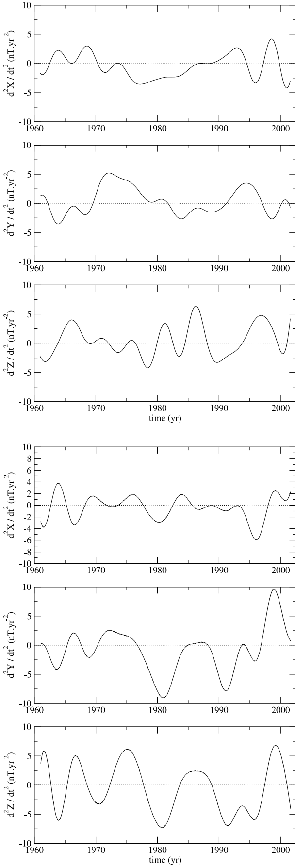
Fig. 1. Secular acceleration, \ddot{X} , \ddot{Y} and \ddot{Z} components, at CLF (Chambon la Forêt, France) observatory ( top ) and API (Apia, Western Samoa) observatory ( bottom ) computed from the CM4 model.
