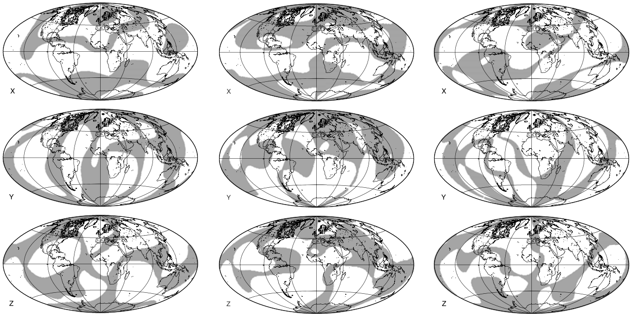
Fig. 3. Maps indicating locations where the zero isoline “swept” the Earth’s surface, so where the geomagnetic jerk appears. From left to right, the three panels correspond to three one-year periods centred onto: 1967.2, 1970.0 and 1972.7, epochs corresponding to the maxima S(t) \geq 5\% .
