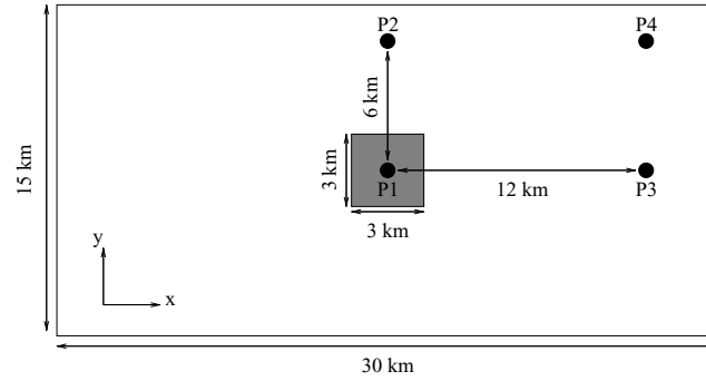
Figure 1. Fault model for testing dynamic rupture simulation for the SCEC problem. The grey square in the centre is the nucleation zone. The black circles are the receivers at which we compare time histories of the shear stress and the slip velocity.
