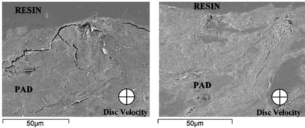
Fig. 13. Superficial cracks develop inside the pad material, after squeal.
