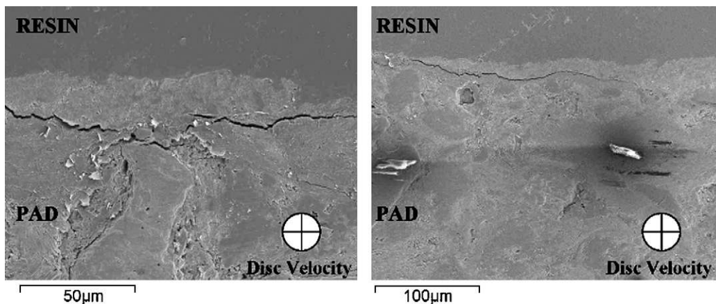
Fig. 11. Section of the pad contact surface normal to the sliding direction, highlighting detachments of the third body layers after squeal.
