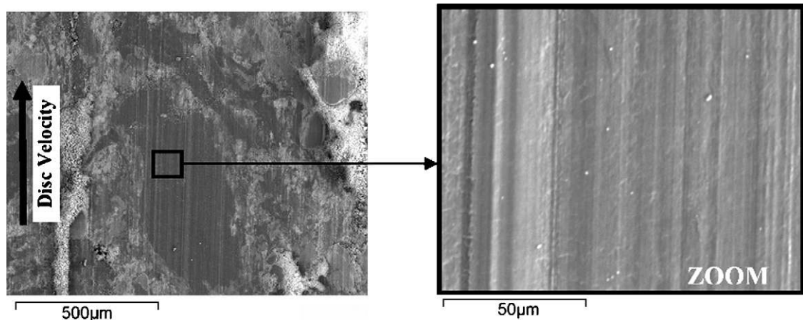
Fig. 6. Contact plateau due to the third body accumulated over the soft pad components (no fibers in the contact area). The third body is compact.
