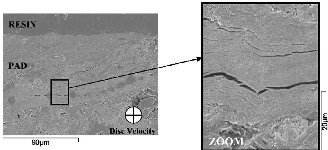
Fig. 14. Internal cracks close to the pad surface developing along layers of pad composites.
