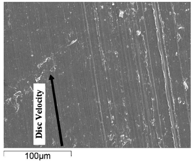
Fig. 10. Disc contact surface; circumferential grooves due to the sliding with the pad.
