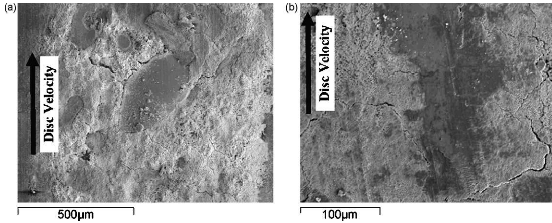
Fig. 9. Superficial cracks both at the no-contact area (a) and at the contact plateaus (b), after squeal.
