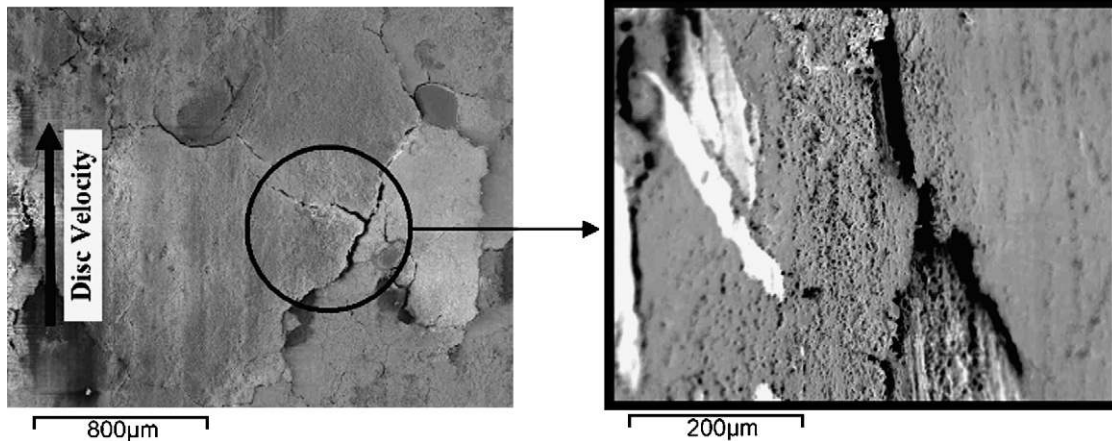
Fig. 7. Material exfoliations at the pad contact surface after squeal.
