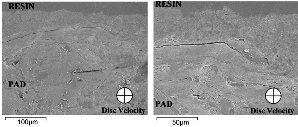
Fig. 12. Detachments of layers of pad material under the third body, after squeal.
