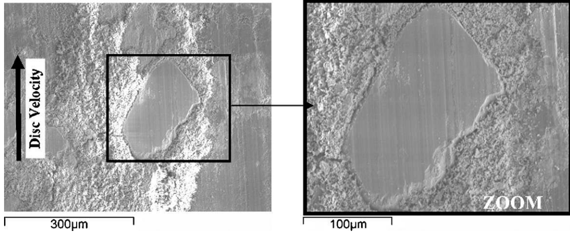
Fig. 5. Contact plateau due to the hard material fiber at the contact surface.
