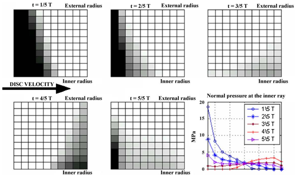
Fig. 4. Contact normal pressure distribution calculated at the pad surface (10 mm × 10 mm) by FEM, for five time steps t along the squeal period T = 2.9e-4 . The average pressure is \bar{\sigma}_n = 1 MPa.
