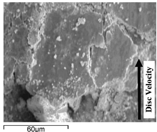
Fig. 8. Micro-exfoliation of the third body (contact plateaus) after squeal.
