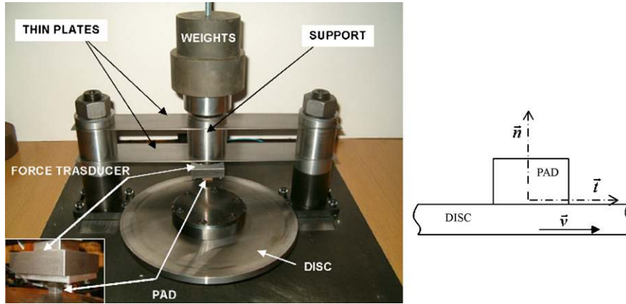
Fig. 1. Left: experimental set-up, TriboBrake COLRIS (Collaboration Lyon-Rome for Investigation on Squeal). Right: schema of the contact.
