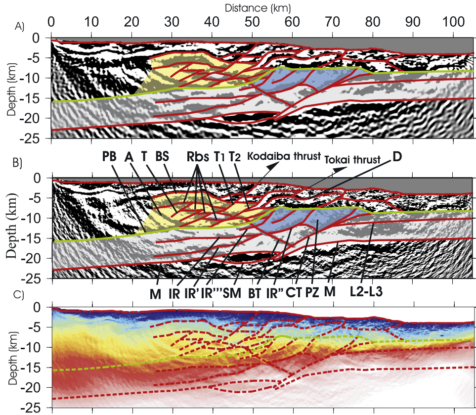
Figure 10. (a) The 3 Hz and (b) 15 Hz perturbation models. (c) Final FWT model. The structural interpretation is superimposed. The gray shaded area delineates the subducting oceanic crust. The blue shaded area delineates the Paleo-Zenisu body on top of the subducting oceanic crust. The yellow shaded area is the backstop. Nomenclatures are M, Moho; BS, top of backstop; Rbs, major reflector in the backstop; T, T1, T2, thrusts affecting the backstop; PZ, Paleo-Zenisu ridge; L2-L3, oceanic layers 2 and 3 of the subducting oceanic crust; D, décollement; Tokai, Tokai thrust; Kodaiba, Kodaiba thrust; CT, thrust affecting the subducting oceanic crust; BT, back thrust; PB, plate boundary (green line) (the plate boundary is assumed to lie on top of the Paleo-Zenisu body); IR, IR', IR'', IR''', intraoceanic crustal reflectors; SM, zone of possibly partially serpentinized mantle; A, artifact; HV, off-scraped high-velocity body.
