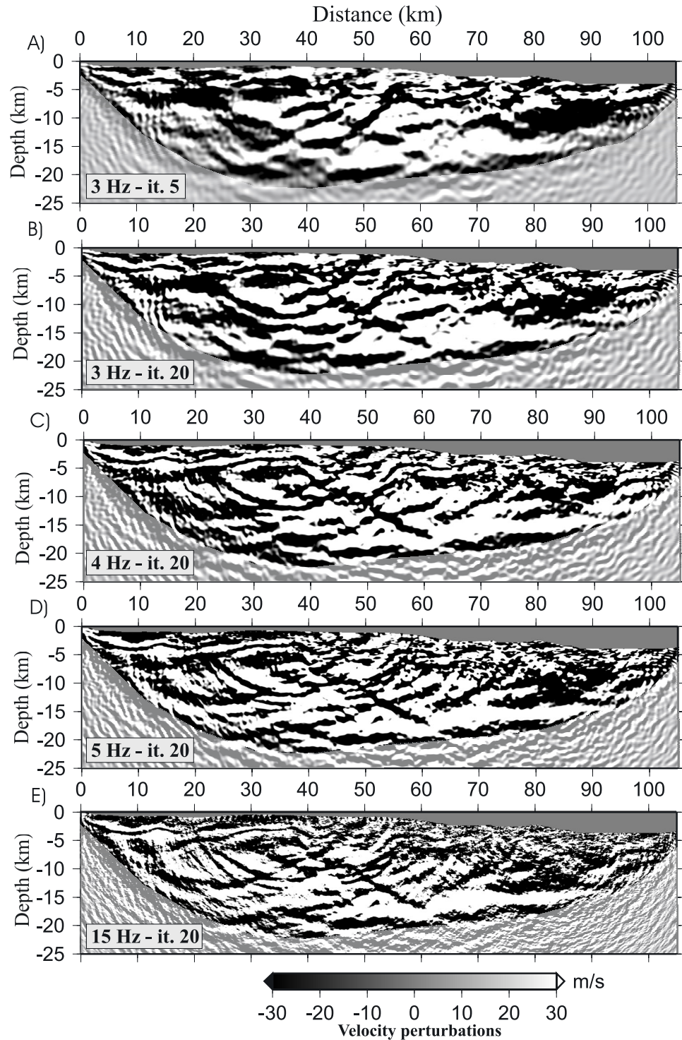
Figure 8. Perturbation models shown with a narrow gray scale spanning between -30 and +30 \text{ m s}^{-1} . (a) Model at 3 Hz, iteration 5. (b) Model at 3 Hz, iteration 20. (c) Model at 4 Hz, iteration 20. (d) Model at 5 Hz, iteration 20. (e) Model at 15 Hz, iteration 20.
