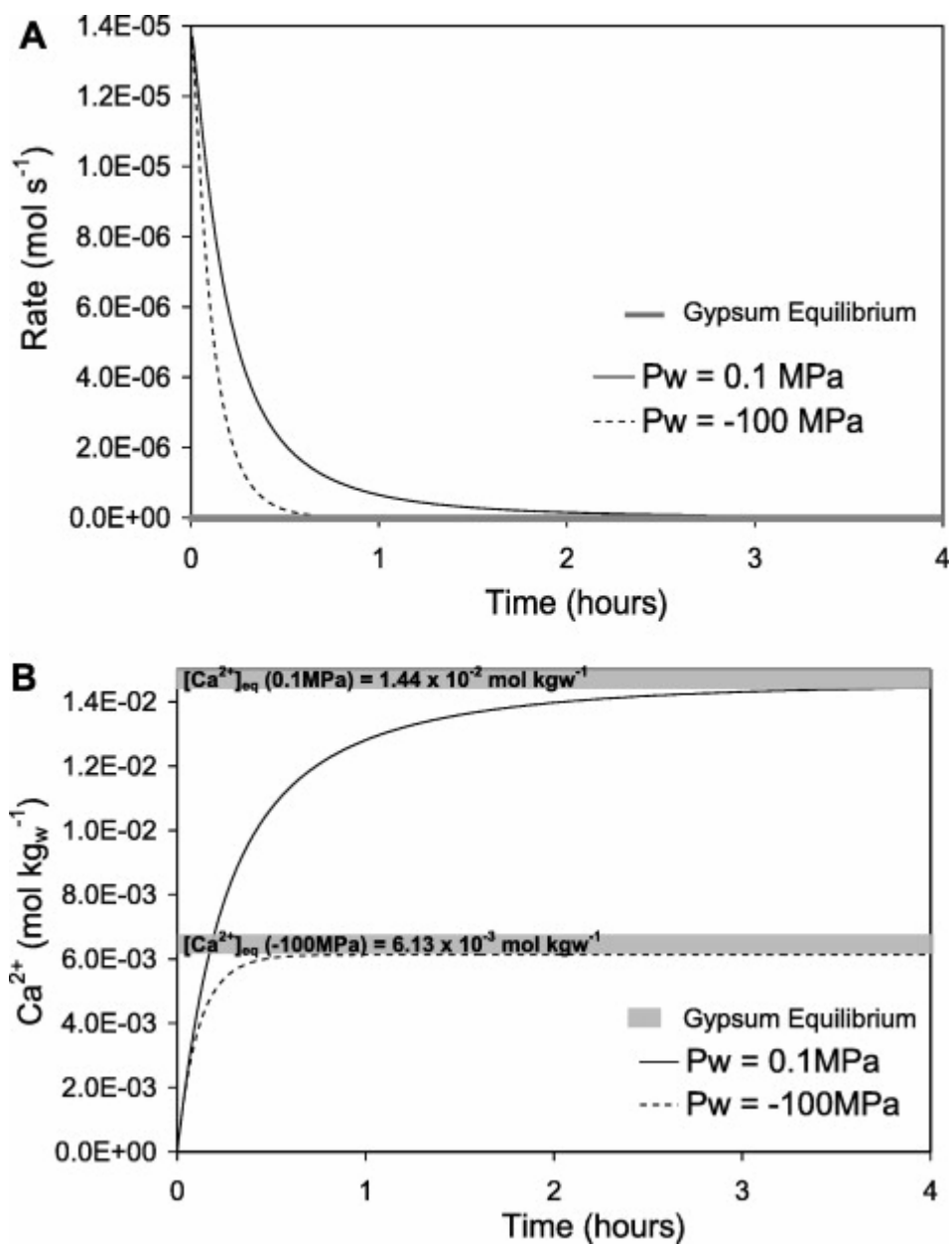
Fig. 7. (A) Gypsum reaction rate ( \text{mol s}^{-1} ) at 25 \text{ }^\circ\text{C} for a solution under -100 \text{ MPa} of pressure and isobaric conditions and under a standard pressure of 0.1 \text{ MPa} . (B) Calcium concentration, from gypsum dissolution, vs. time.
