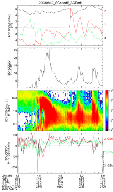
Figure 1. ACE-MFI and CIS-CODIF (spacecraft 4) data with, from top to bottom, the shifted interplanetary magnetic field, the proton density, a proton energy-time spectrogram, and the proton velocity.
