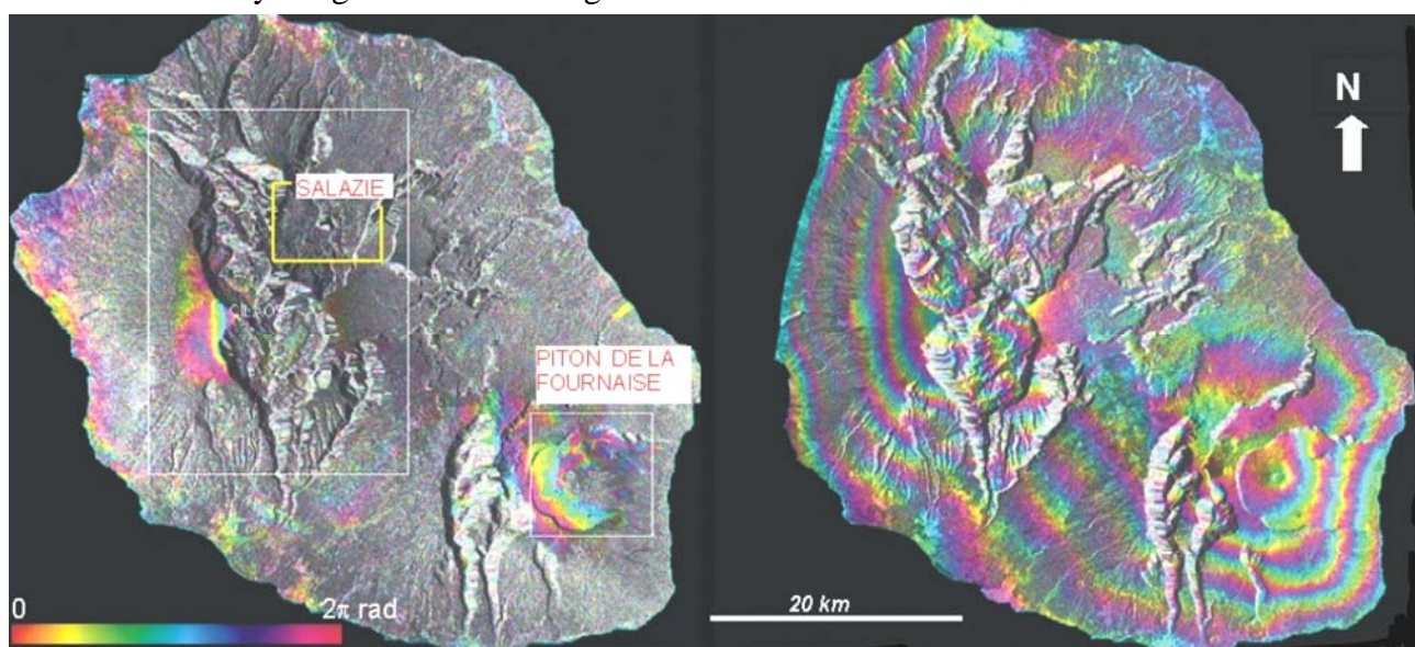
Figure 1. Left: one of the most coherent Radarsat C-band interferograms (15/05/2001 – 23/11/2001, perpendicular baseline=68 m). Right: one of the most coherent JERS-1 (02/01/1997–14/05/1997, perpendicular baseline=187 m) interferograms obtained for the whole island. The white rectangles on Figure 1 indicate the Circles sector and the Piton de la Fournaise volcano. The yellow rectangle shows the area displayed in Figure 2. No coherence loss is observed in the L-band despite the dense vegetal cover of the island. The SAR intensity image is used as background.
