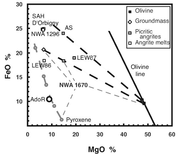
Fig. 10. FeO:MgO diagram. Mass balance permits to derive possible groundmass composition once the bulk rock and olivine compositions are known. Notice that angrites with olivine xenocrysts (picritic angrites) are significantly enriched in MgO relative to pure angritic melts like D'Orbigny. AdoR (Angra dos Reis) a pyroxene cumulate and the pyroxene compositions of NWA 1670, suggest that different angrites relate to one another through pyroxene accumulation.
