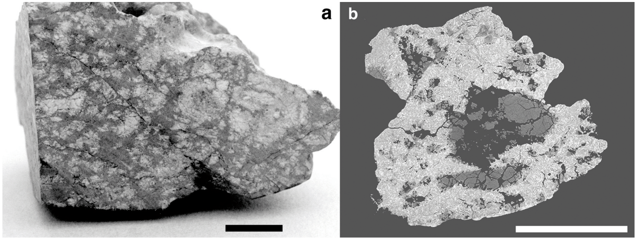
Fig. 1. a) View of the sawn surface showing the abundant olivine xenocrysts surrounded by the dark matrix; scale bar 5 mm. b) Composite BSE image showing the whole section studied in this report; scale bar 5 mm. Notice the large olivine crystals in the center (light gray) partly lost during sample preparation.
