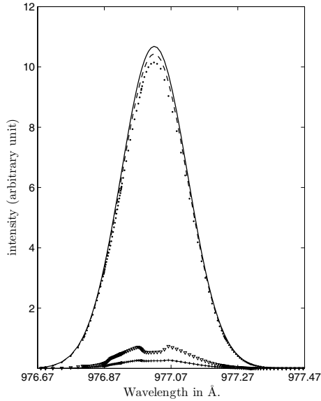
Fig. 5. Stellar C III line in a situation just before an transit (solid line) and during the transit with an H 2 layer 25 000 km thick (dashed line) and with an H 2 layer 100 000 km thick (dotted line). The wavelength centre of the C III line is at 977.02 Å. The bottom lines represent the difference between the two curves (25 000 km for the crosses, 100 000 km for the triangles).
