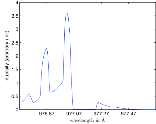
Fig. 6. Emission of the planet in the region of the C III line in a geometry similar to the Fig. 4, i.e. with a maximum angular separation.
