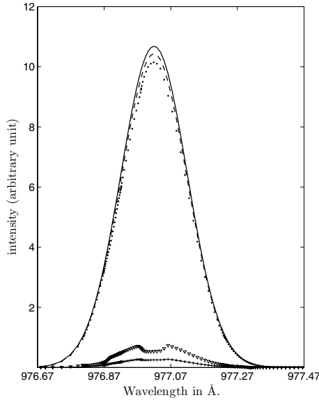
Fig. 5. Stellar C III line in a situation just before a transit (solid line) and during the transit with an H 2 layer 25 000 km thick (dashed line) and with an H 2 layer 100 000 km thick (dotted line). The wavelength centre of the C III line is at 977.02 Å. The bottom lines represent the difference between the two curves (25 000 km for the crosses, 100 000 km for the triangles).
