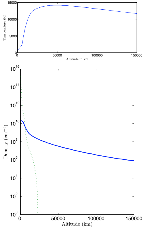
Fig. 1. HD 209458b atmospheric model. Upper panel: temperature profile in the atmosphere of the planet HD 209458b; from Yelle (2004). Lower panel: density profiles of H (solid line) and H 2 (dashed line) in the atmosphere of HD 209458b; from Yelle (2004).
