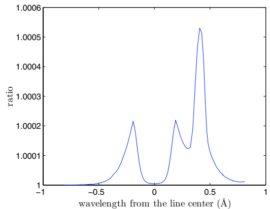
Fig. 3. Ratio of the Lyman \alpha line profile during a transit with the H 2 layer divided by the line profile without the H 2 layer.
