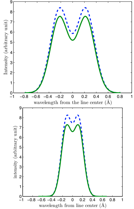
Fig. 2. Lyman \alpha (upper panel) and Lyman \beta (lower panel) line profile from the star with or without a transit with a 25 000 km thick H 2 layer. The diminution of the total intensity is 10.45% in the Lyman \alpha case, and 10.53% in the Lyman \beta case. The difference is consistent with the fact that Lyman \beta has a single scattering albedo equal to 0.86 lower than the Lyman \alpha single scattering albedo, equal to 1. No effect of the H 2 lines is visible.
