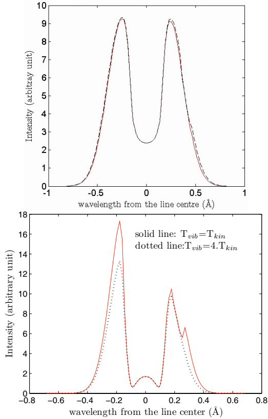
Fig. 4. Planetary emission in the Lyman \alpha (upper panel) and Lyman \beta cases (lower panel) for several vibrational temperatures (1 and 4 times the kinetic ones). The lack of symmetry is very faint in the case of Lyman \alpha and strong in the case of Lyman \beta . In the two panels, the solid line corresponds to T_{\text{vib}} = T_{\text{kin}} . The dotted line corresponds to T_{\text{vib}} = 4T_{\text{kin}} .
