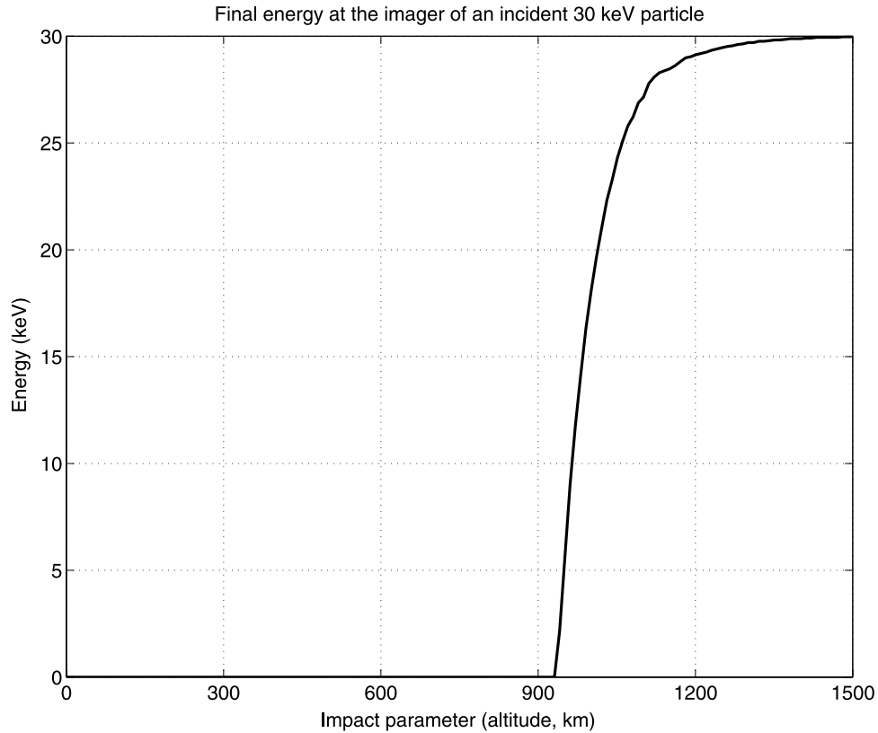
Figure 5. Final energy of an incident 30 keV particle (ion or ENA) when it reaches the imager, after eventually multiple charge transfer collisions (process nos. 1, 2, 3).
