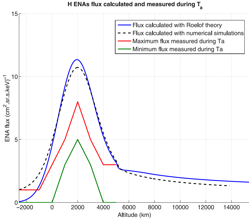
Figure 6. Comparison between the simulations and the measurements for the ENA profiles during the Ta flyby for an altitude of about 8000 km and energies between 20 and 50 keV. We show here the reprocessed INCA data (minimum and maximum in green and red, the simulations with the Roelof formalism (blue) and a two-dimensional numerical model (dashed black). See text for more details.
