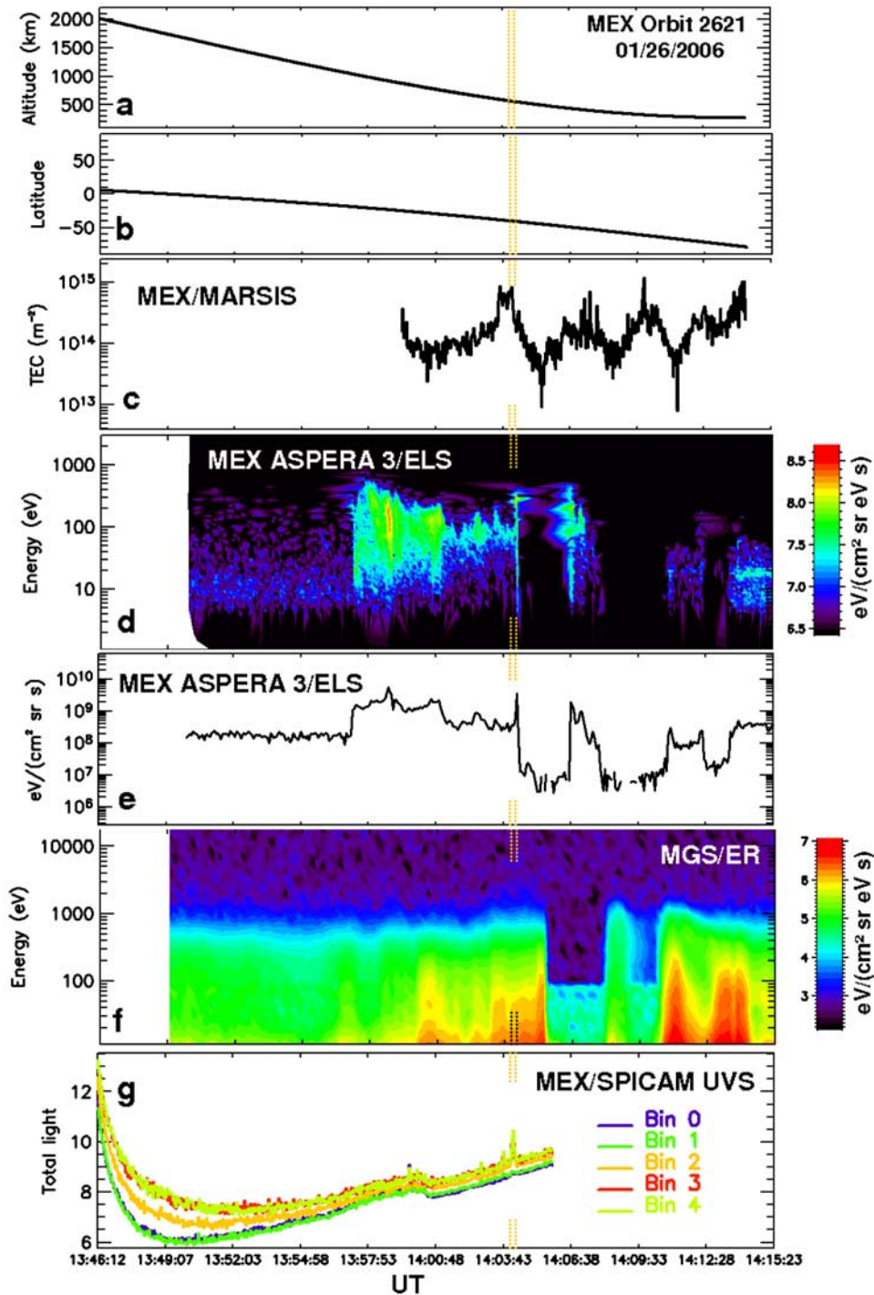
Figure 4. Time series of the measurements during orbit 2621. Shown is the MEX (a) altitude and (b) latitude, (c) MEX/MARSIS Total Electron Content, (d) MEX/ASPORA-3/ELS sector 1 (which is the sector facing the zenith) electron measurement in \text{eV}/(\text{cm}^2 \text{sr eV s}) , (e) MEX/ASPORA-3/ELS energy flux of sector 1, (f) MGS/MAG-ER electron energy flux averaged over the full set of sectors in \text{eV}/(\text{cm}^2 \text{sr eV s}) , and (g) MEX/SPICAM UVS measurements summed over the full spectral range for each spatial bin in ADU. Indicated on each by vertical dotted lines are the periods during which an aurora event has been identified in SPICAM UV observations.
