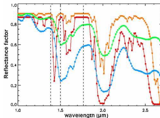
Figure 4.1.: model spectra of CO 2 ice with grains of 1 mm (orange) and 5 cm (red), and H 2 O ice with grains sizes of 10 \mu m (green) and 1000 \mu m (blue). The three dashed lines correspond to the OMEGA spectels at 1.385 \mu m, 1.5 \mu m and 1.77 \mu m which are used for the determination of the strength of the H 2 O ice absorption at 1.5 \mu m, as this is the only weak CO 2 absorption at these wavelengths.
