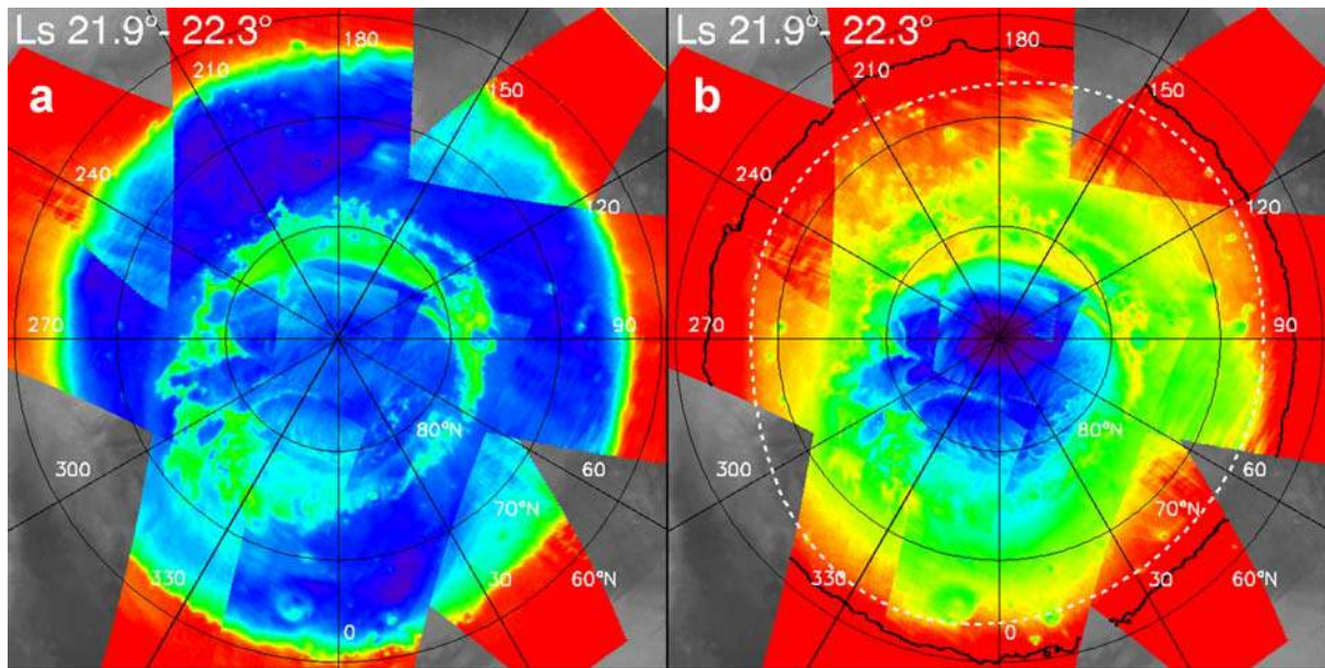
Figure 4.2: seasonal evolution of the northern polar cap: spatial distribution of spectral signatures of H 2 O ice and CO 2 ice observed by OMEGA in early northern spring (Ls 22°, March 2006). a) band depth of the H 2 O ice absorption feature at 1.5 μm. The rainbow scale covers the range from 60% (black) to 0% (red); b) band depth of the CO 2 ice absorption feature at 1.43 μm, also from 60% (black) to 0% (red). The annulus observed by TES between the boundary of bright regions (black line on panel "b") and that of regions at the equilibrium temperature of CO 2 ice (crocus line, white dashes, from Titus and Kieffer, 2003) is confirmed as being constituted of H 2 O frost. At this season, the strongest CO 2 ice signatures, corresponding to large mean grain sizes, are observed over regions corresponding to the central parts of the North permanent cap.
