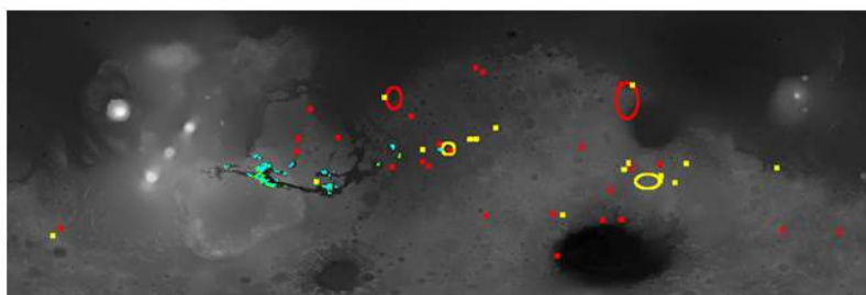
Figure 7.1.: distribution of hydrated minerals detected so far by OMEGA at the surface of Mars, for latitude from -50^\circ to +50^\circ . Blue: kieserite; green: polyhydrated sulfates; red: phyllosilicates; yellow: other hydrated minerals.
