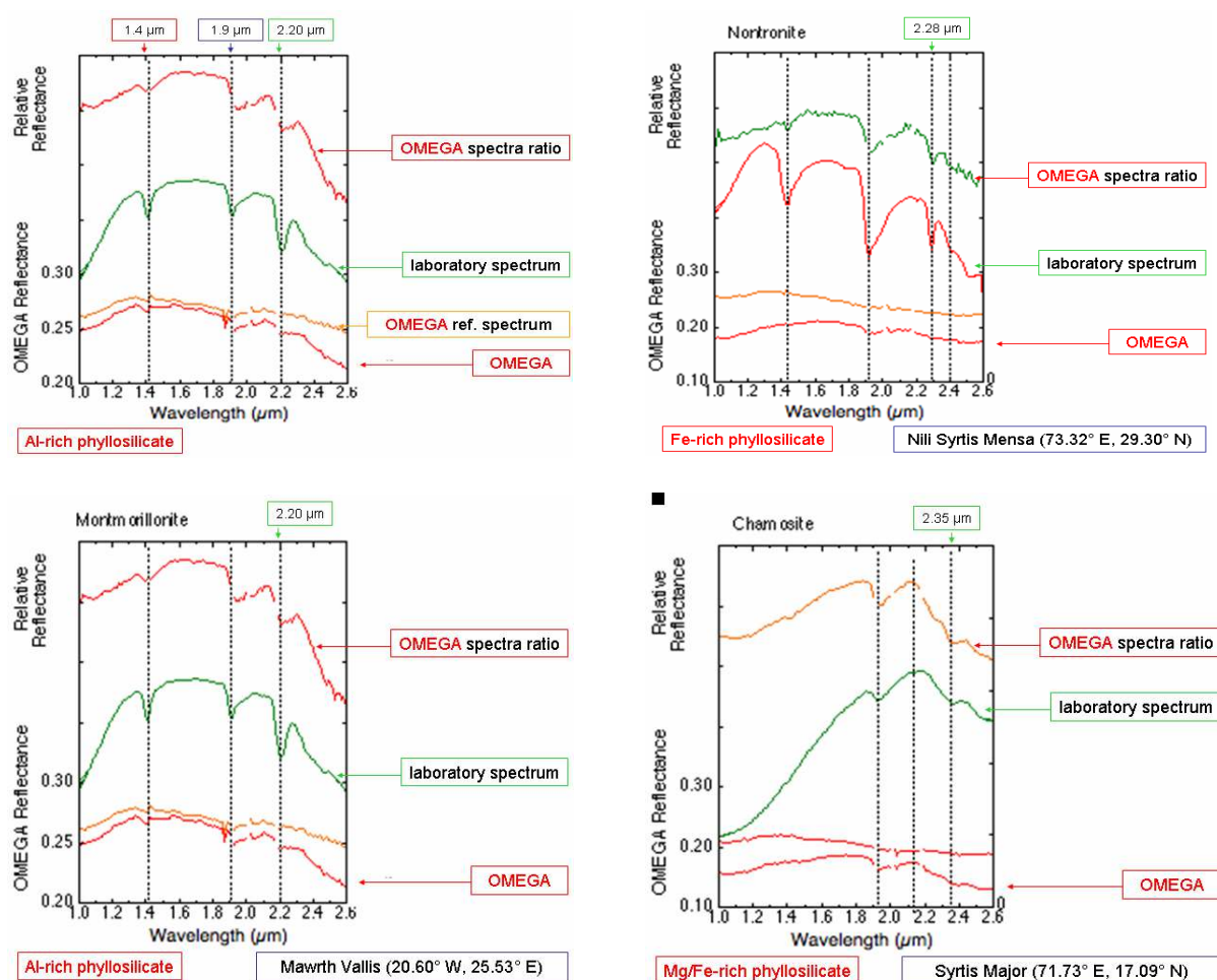
Figure 7.7.: spectra of hydrated phyllosilicates, as detected by OMEGA, compared to laboratory spectra, showing the diagnostic shift of the M-OH feature from 2.2 \mu\text{m} for Al-rich (a,b) to 2.28 \mu\text{m} Fe-rich (c) and 2.35 \mu\text{m} Mg/Fe-rich (d) species.
