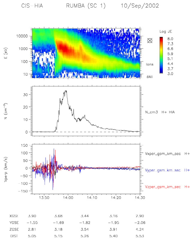
Fig. 1. Example of dispersed cusp under Southward IMF. From top to bottom: ion time-energy spectrogram, number density and convection velocity in GSM from Cluster-CIS.
