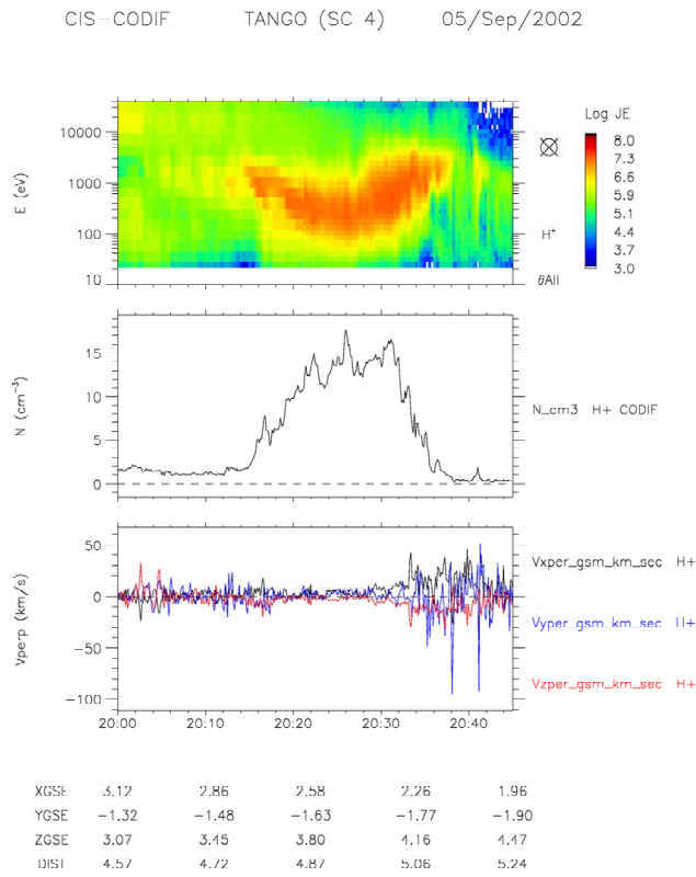
Fig. 3. Example of discontinuous cusp. From top to bottom: ion time-energy spectrogram, number density and convection velocity in GSM from Cluster-CIS.
