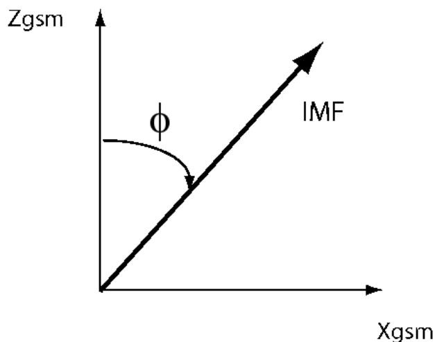
Fig. 9. Definition of the cone angle ( \phi ).
