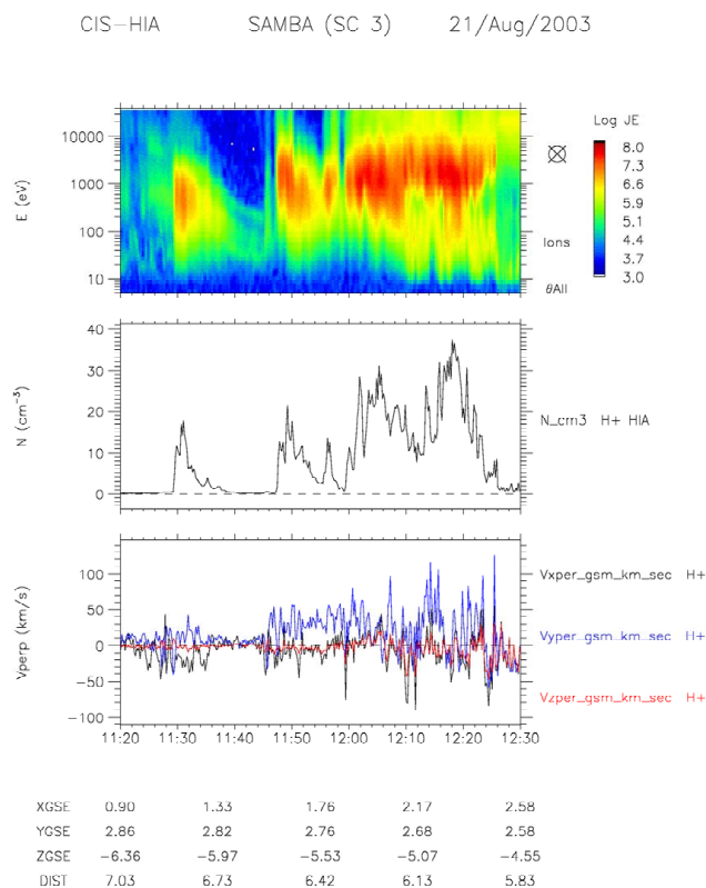
Fig. 4. Example of irregular cusp. From top to bottom: ion time-energy spectrogram, number density and convection velocity in GSM from Cluster-CIS.
