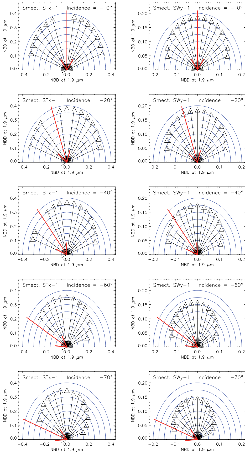
Figure 7. Polar plots of the 1.9\text{-}\mu\text{m} band NBD parameter values calculated for the two smectites. (left column) Smectite STx-1 (laboratory measurements). (right column) Smectite SWy-1 (model with d = 20 \mu\text{m} and g = 0.4 ). Each row corresponds to a different incidence angle ( 0^\circ , 20^\circ , 40^\circ , 60^\circ , 70^\circ from top to bottom).
