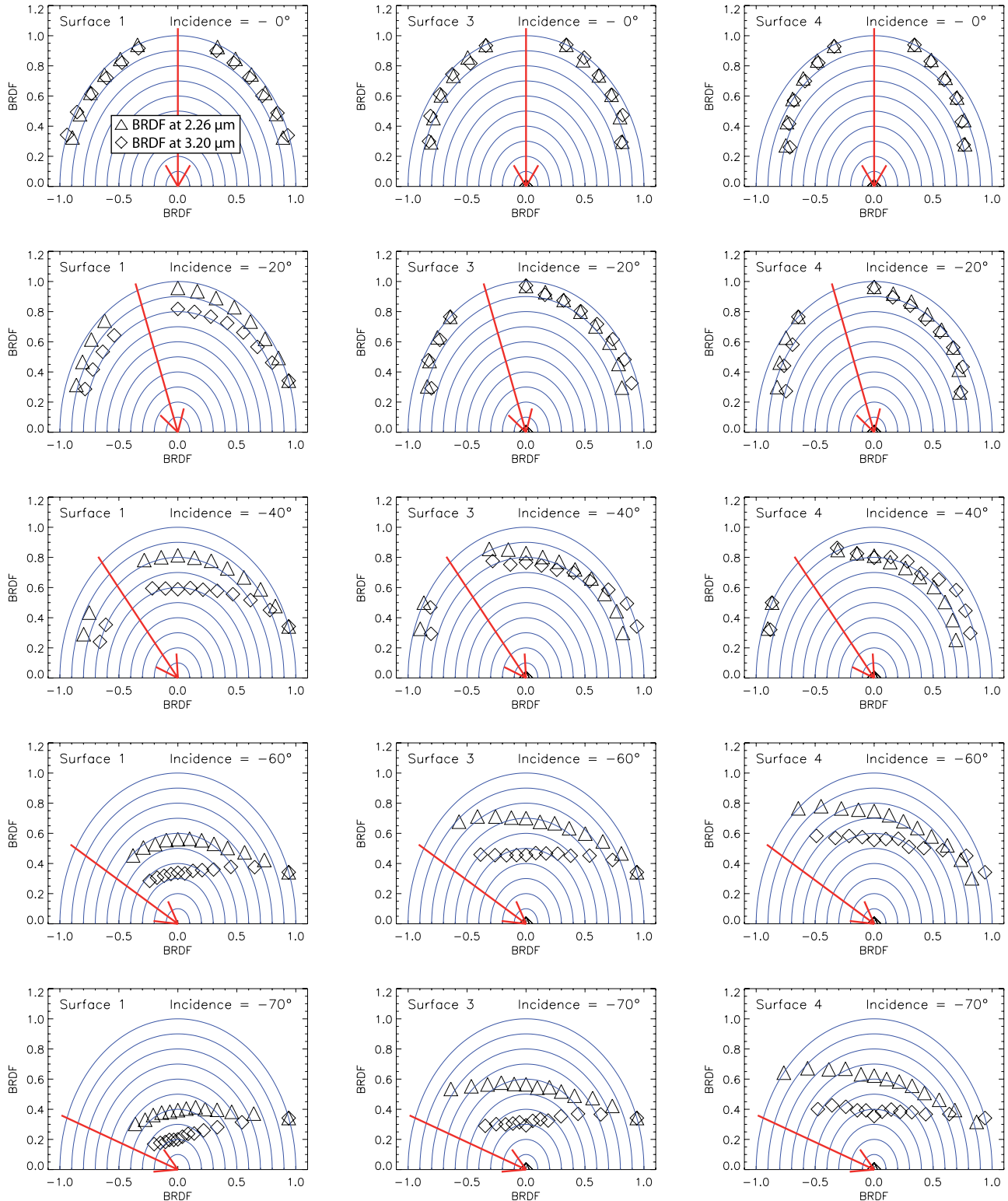
Figure 16. Comparison of BRDF behaviors in the continuum ( 2.26 \mu\text{m} ) and in the 3.2 \mu\text{m} absorption band for the three different surfaces prepared with the volcanic tuff. Each BRDF is normalized to 1 at its maximum value for a better comparison of the BRDF shapes and evolutions. (left column) Smooth surface prepared with ( 50-100 \mu\text{m} ) fraction. (center column) Smooth surface + 0.32 \text{ g} of large grains (fraction [800-1120 \mu\text{m}] ). (right column) Smooth surface + 0.52 \text{ g} of large grains. Each row corresponds to a different incidence angle ( 0^\circ , 20^\circ , 40^\circ , 60^\circ , 70^\circ ) indicated by the arrow.
