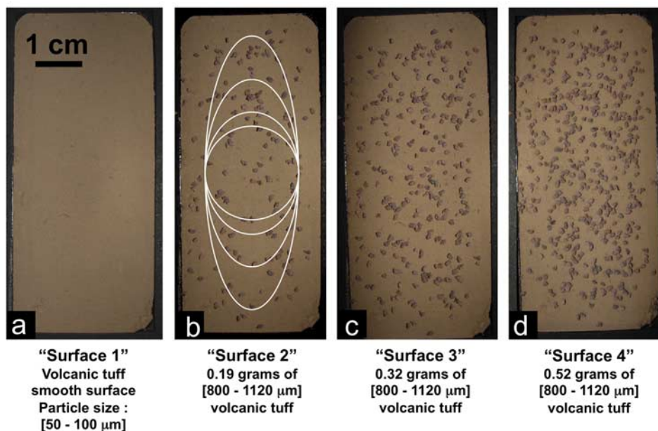
Figure 1. Synthetic image consisting in four photographic images of different surfaces prepared with two particle size fractions of the volcanic tuff sample: [50–100 \mu\text{m} ] and [800–1120 \mu\text{m} ]. (a) Smooth surface prepared with the small grain fraction. (b to d) Successive additions of large volcanic tuff grains on the smooth surface presented in Figure 1a. Figure 1b also illustrates the areas of the surface seen by the detectors at different emission angles. The circle in the center (2-cm diameter) corresponds to observations at nadir (emission angle = 0^\circ ). The three ellipses correspond to successive emission angles of 40^\circ , 60^\circ and 70^\circ (from the smallest to the largest one).
