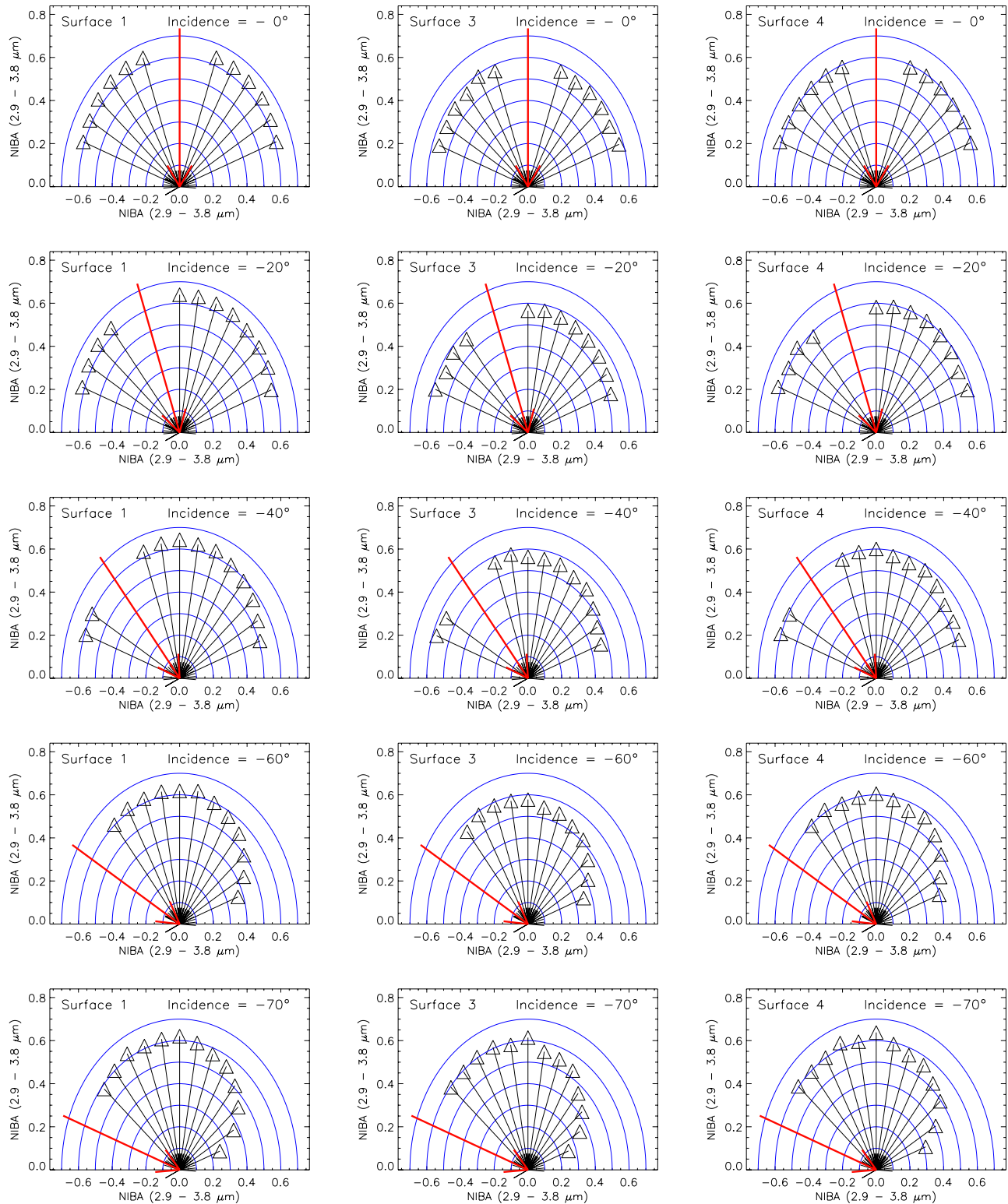
Figure 15. Polar plots of NIBA at 3 \mu\text{m} for three different surfaces prepared with the volcanic tuff. (left column) Smooth surface prepared with (50\text{--}100 \mu\text{m}) fraction. (center column) Smooth surface + 0.32 \text{ g} of large grains (fraction [800\text{--}1120 \mu\text{m}] ). (right column) Smooth surface + 0.52 \text{ g} of large grains. Each row corresponds to a different incidence angle ( 0^\circ , 20^\circ , 40^\circ , 60^\circ , 70^\circ ) indicated by the arrow.
