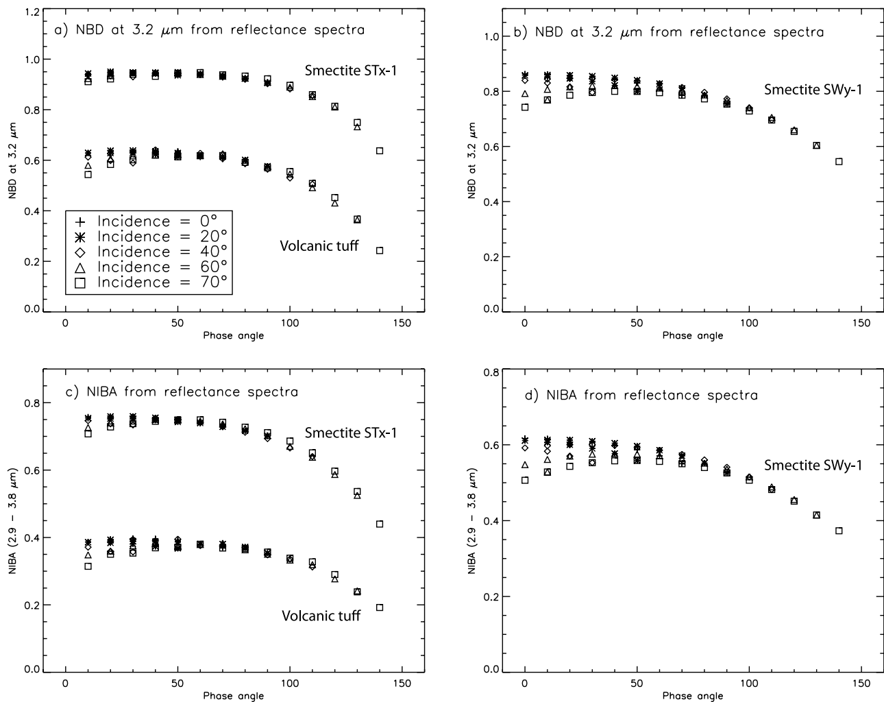
Figure 10. Evolution of the 3\text{-}\mu\text{m} band strength as a function of phase angle. (a and c) Experimental results for the STx-1 smectite (top trace in each plot) and the volcanic tuff (bottom trace). (b and d) Results from radiative transfer modeling for the SWy-1 smectite ( d = 20\ \mu\text{m} and g = 0.4 ). Different symbols are used to distinguish series of measurements made with different incidence angles (see legend on Figure 10a).
