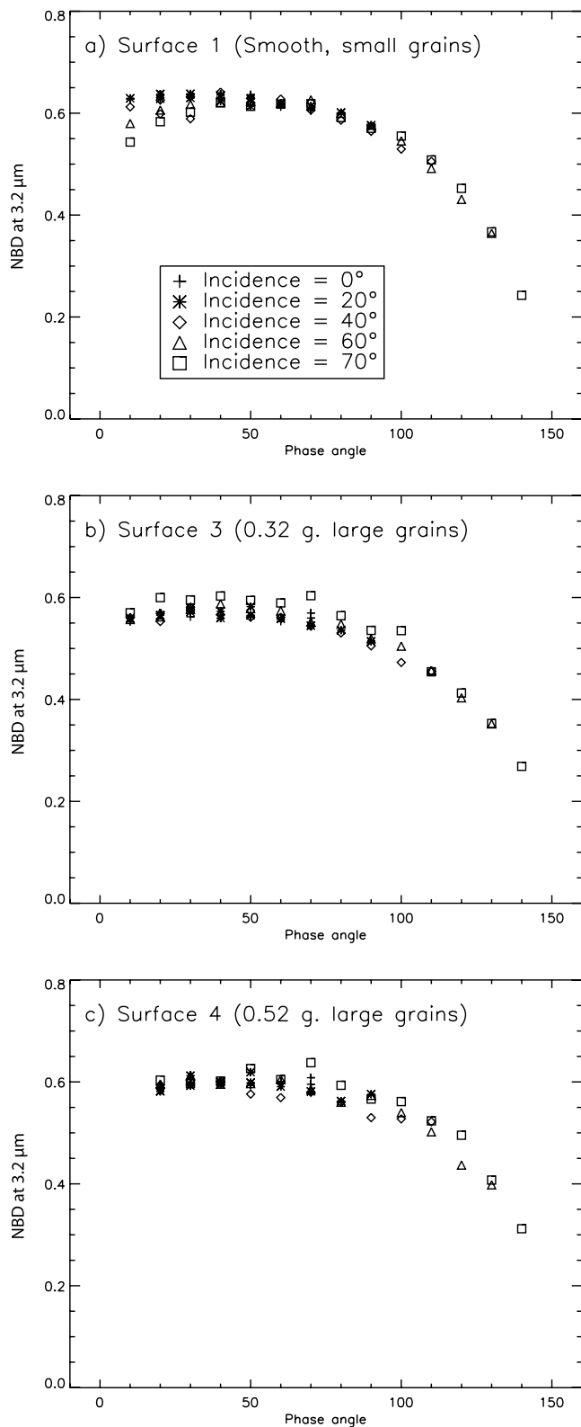
Figure 17. Evolution of NBD at 3.2 \mu\text{m} as a function of phase angle for three different surfaces prepared with volcanic tuff. (a) Smooth surface prepared with the [50\text{--}100 \mu\text{m}] fraction. (b) Smooth surface + 0.32 g of large grains (fraction [800\text{--}1120 \mu\text{m}] ). (c) Smooth surface + 0.52 g of large grains.
