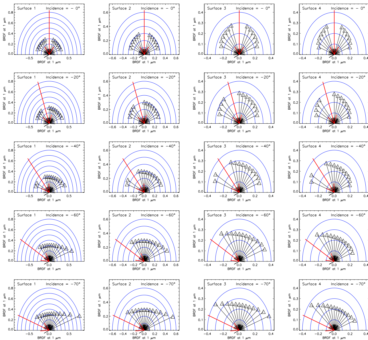
Figure 14. BRDF polar plots at 1 \mu\text{m} for the four different surfaces prepared with the volcanic tuff ( 50\text{--}100 \mu\text{m} ) and ( 800\text{--}1120 \mu\text{m} ) particle size fractions. See Figure 1 for pictures and description of these surfaces. Each column corresponds to a different surface (progressive addition of large grains on smooth surface from left to right). Each line corresponds to a different incidence angle ( 0^\circ , 20^\circ , 40^\circ , 60^\circ , 70^\circ ) indicated by the arrow. The effect of adding large grains on the smooth surface is a transition from a forward scattering behavior to a backscattering behavior due to the appearance of shadows at high phase angle.
