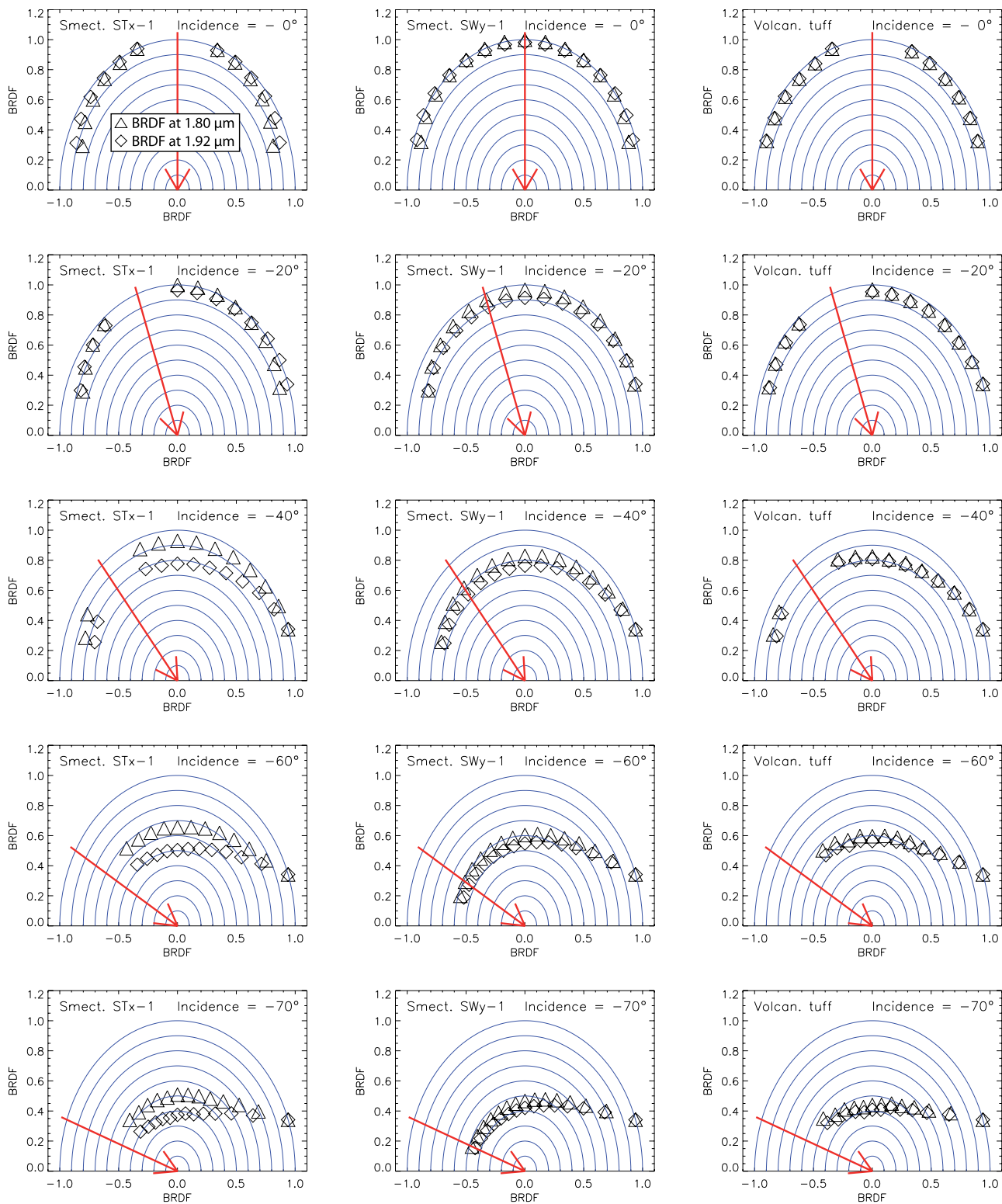
Figure 9. BRDF polar plots for the three smooth surfaces. BRDF is plotted at two different wavelengths: 1.80 \mu\text{m} (continuum) and 1.92 \mu\text{m} (minimum in the 1.9\text{-}\mu\text{m} absorption band). To allow for a better comparison between the BRDF shapes, BRDF at each wavelength is normalized by its maximum value. (left column) Smectite STx-1 (laboratory measurements). (center column) Smectite SWy-1 (model with d = 20 \mu\text{m} and g = 0.4 ). (right column) Volcanic tuff (Laboratory measurements). Each row corresponds to a different incidence angle ( 0^\circ , 20^\circ , 40^\circ , 60^\circ , 70^\circ from top to bottom).
