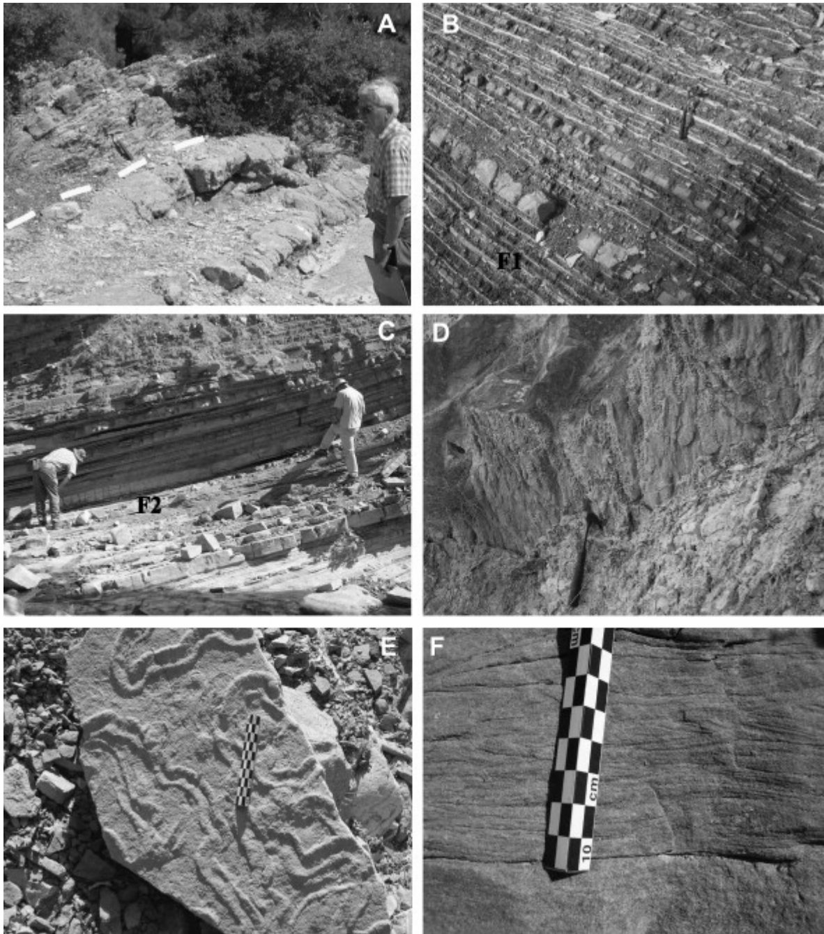
Fig. 6. (A) Field view of algal limestones of the Karabayır formation (Aquitania) unconformably overlying Upper Cretaceous pelagic limestones. The dash line shows the boundary (location on Fig. 4a, section 2). (B) Field view of facies F1 showing alternating mudstone–sandstones and micritic carbonates. Hammer for scale. (C) General appearance of facies F2 with siltstone-fine sandstone alternations. (D) Flute casts developed under the calcareous sandstone beds. (E) Trace fossils on top of a calcareous sandstone bed. (F) Fine ripples developed on top of calcareous sandstone (Bouma Tc division).
