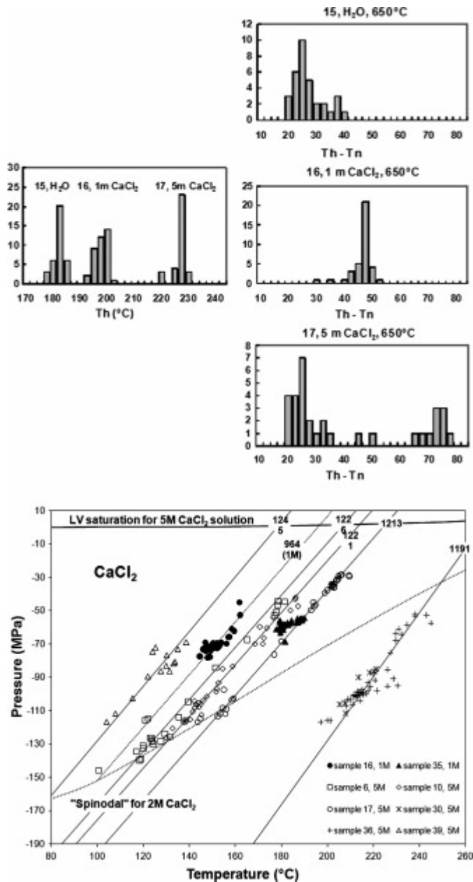
Fig. 5. Micro-thermometric data (upper) and P - T coordinates (lower) of 229 \text{CaCl}_2 (1 and 5 M) fluid inclusions (8 samples) trapped in quartz. Each isochore is labeled with the liquid density in \text{kg m}^{-3} .
