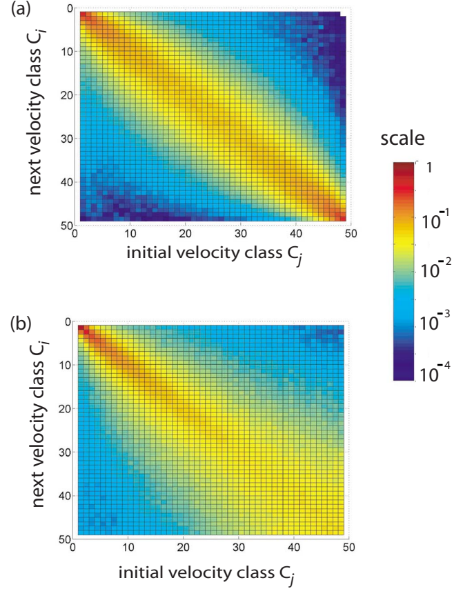
FIG. 7. (Color online) Transition matrix in distance \mathbf{T}^s(\lambda/2) for the multilognormal field and the connected field.
