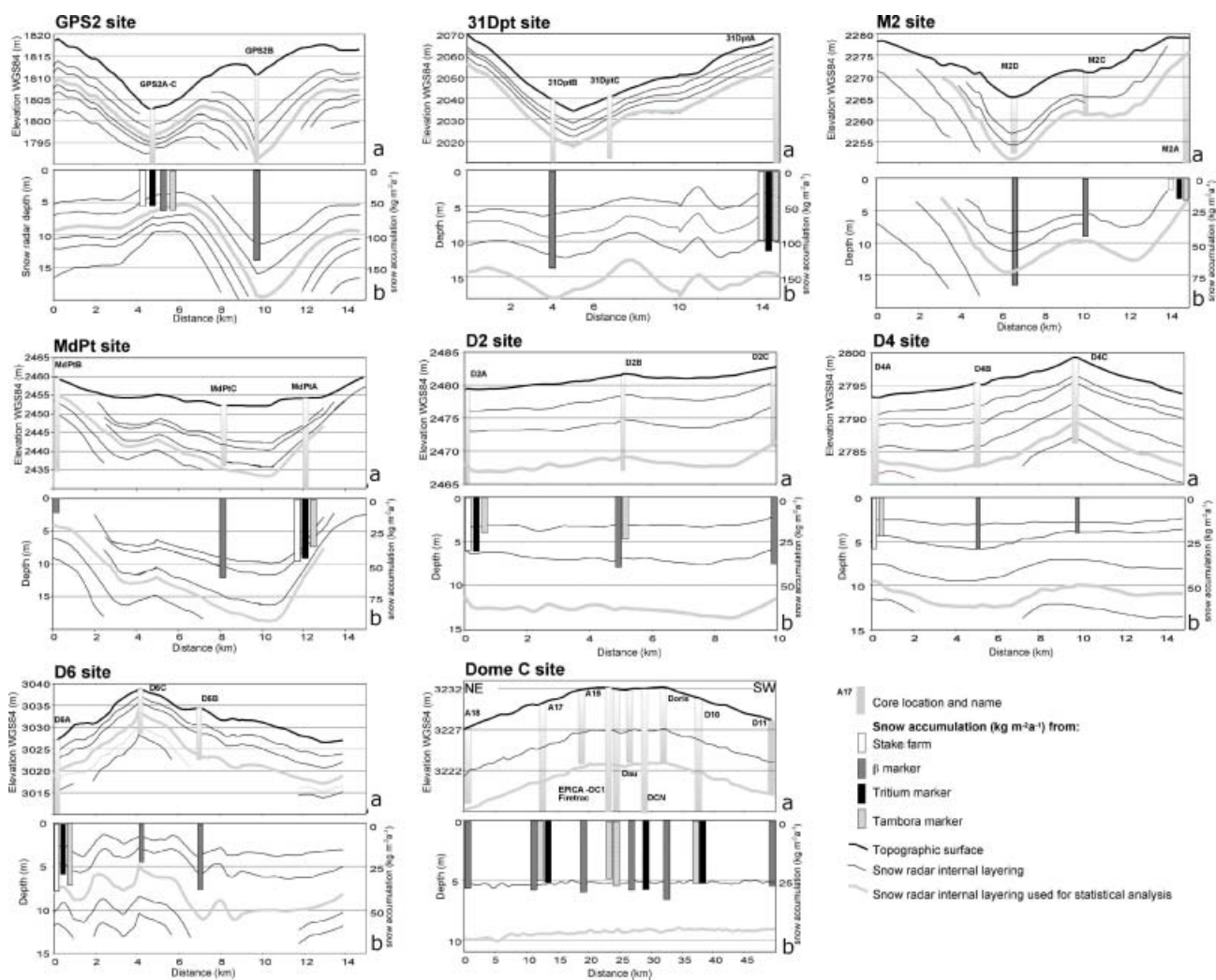
Fig. 2. (a) Core location and elevation of GPR selected horizons and surface profiles; (b) depth profile of GPR selected horizons and snow accumulation from firn cores using different methods.
