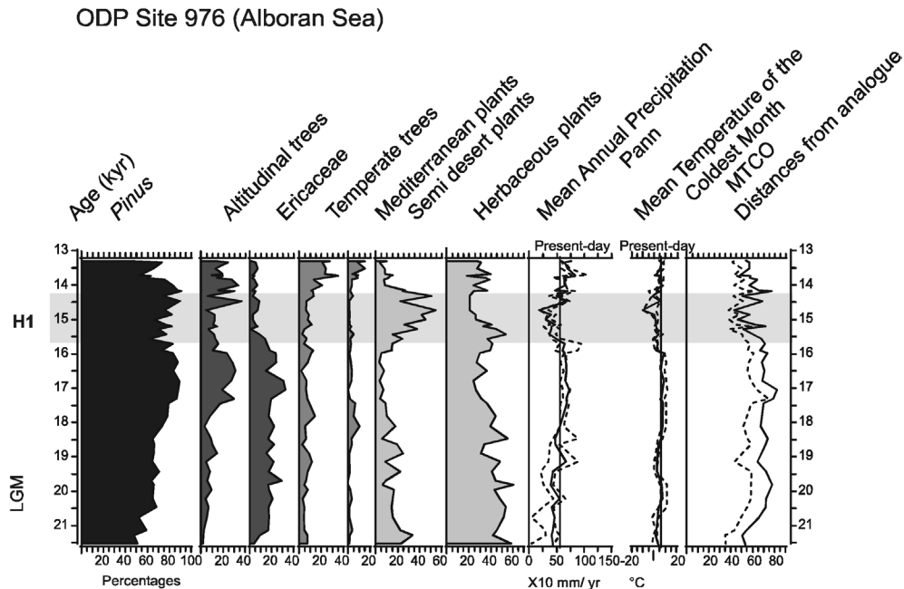
Fig. 1. First 7 curves: simplified pollen diagram for ODP site 976. Percentages for taxa other than Pinus are computed from a pollen sum excluding Pinus . Curves 8 and 9: Reconstruction of the annual precipitation and mean temperature of the coldest month. Dotted curves indicate minimum and maximum reconstructions. Last curve: Similarity index (Chord distance) measuring the quality of the modern analogues. The figure shows the calculated distance of the first (dotted line) and the last (solid line) of the best analogues selected.
