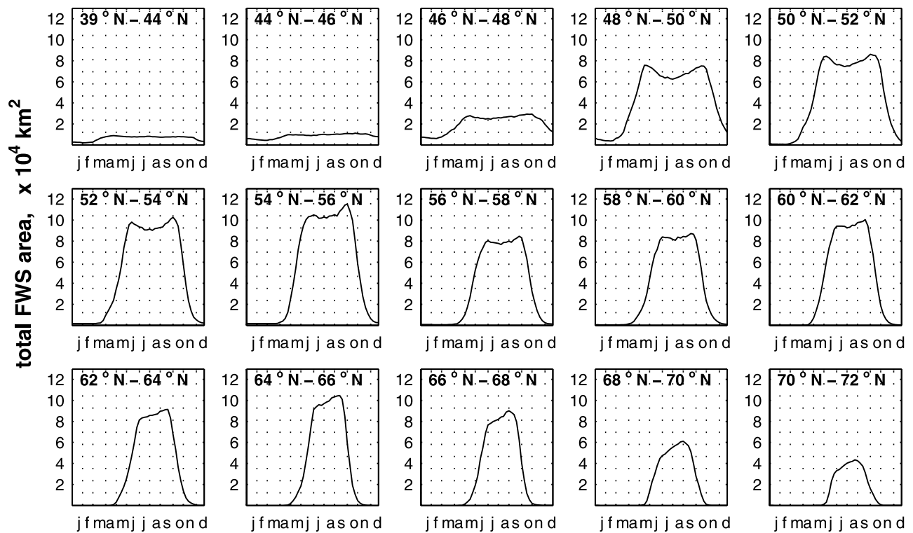
Figure 5. Latitudinal variation (every 2^\circ , except for southern latitudes, 39^\circ\text{N} – 44^\circ\text{N} , where FWS are small) of the seasonal dynamics of the wetland and waterbody extent (total fraction of water surface area \times 10^4 \text{ km}^2 ) over Canada-Alaska for the 1988–2001 period.
