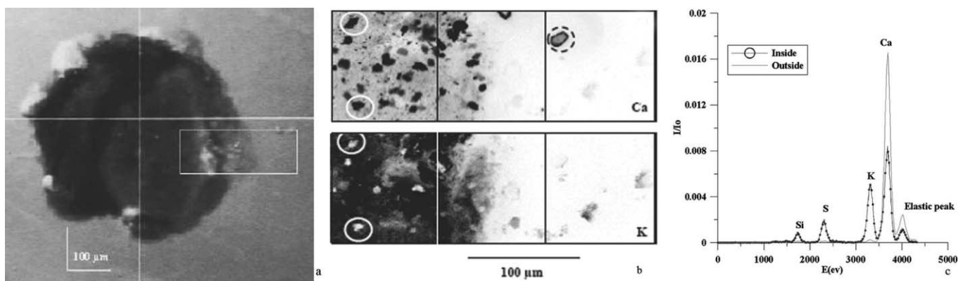
Fig. 6. (a) Aggregate observed on the V1 sample (Vostok at 3551 m). The lighter regions (visible at the periphery) may be gas bubbles, while the dark regions look like the solid part of the aggregate. The rectangular region indicated was analyzed by \mu XRF. (b) Results of the analysis: maps of Ca and K distributed on the aggregate (image size 300 \times 100 \mu\text{m}^2 ; pixel size: 1 \times 1 \mu\text{m}^2 ; integration time 0.5 s). Ca is distributed as large particles. Their shapes and compositions are different inside (circles) and outside (dashed circle) the aggregate. Ca seems anticorrelated with K (white circles). (c) \mu XRF spectra from the upper particles inside and outside the aggregate (circled in (b)).
