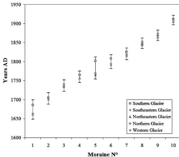
Fig. 4. Dates obtained for the ten main moraines of the five Charquini glaciers. Dates obtained from lichen size measurements are generally consistent from one glacier to another. The discrepancy for the moraines M5 and M6 of the southern glacier can be attributable to insufficient sampling lichen measurements, since the moraines found in that sites are made up of fine-grained materials. For M1 moraine on the same glacier, although a problem in the lichen sampling cannot be ruled out, this glacier might reach its maximum size some decades later or stay in the same position for a longer period. Cumulative error margins are illustrated.
