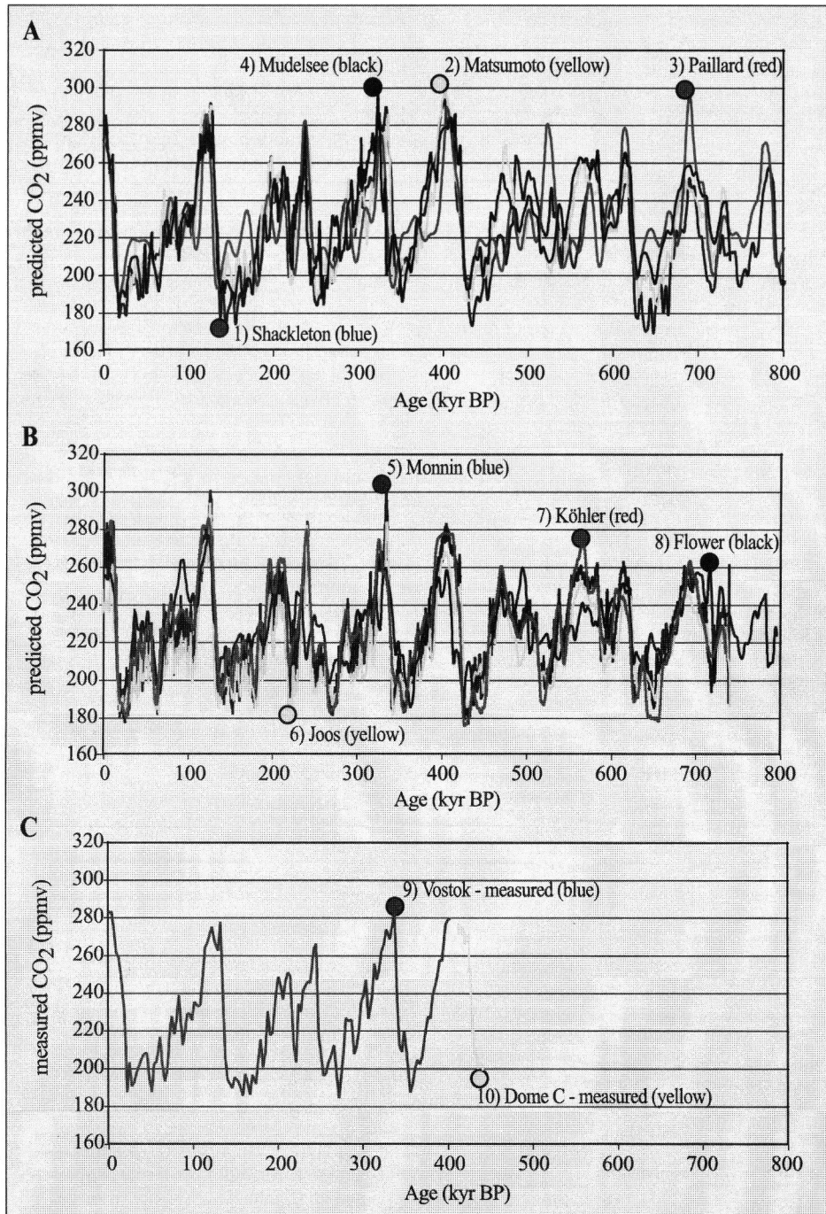
Fig. 1. (a and b) Predictions of \text{CO}_2 concentration over the past 740 kyr, labeled with the name of the respective lead author. (c) \text{CO}_2 concentrations measured in ice cores. The Vostok data are on the timescale known as GT4 [Petit et al., 1999]; the small amount of additional data published so far from the EPICA Dome C core (EDC2 timescale) are included [EPICA Community Members, 2004]. The two timescales have a small mismatch at the period of overlap between the two records, but this presentation allows the changes in \text{CO}_2 occurring at the glacial/interglacial transition known as Termination V, about 430 kyr B.P., to be seen.
