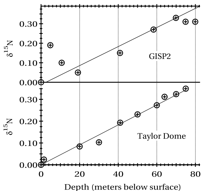
Figure 1. Firm air \delta^{15}\text{N} profiles from GISP2 and Taylor Dome. The solid lines show the expected increase calculated using the barometric equation (equation (1)). The line on the GISP2 plot, drawn through the two deepest points in the diffusive zone (57 and 70 m), extrapolates to zero \delta^{15}\text{N} at 2 m depth, indicating a convective zone of this thickness. The \delta^{15}\text{N} values are reported in per mil. Analytical errors are smaller than the symbols.
