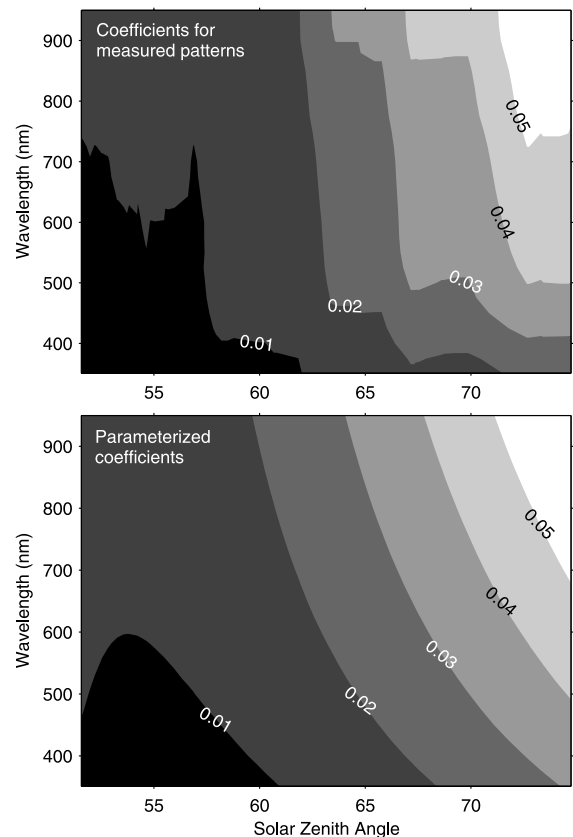
Figure 10. Contour plots of the coefficients multiplying the first EOF of the data in parameterization A. (top) Coefficients fitting the measured data, smoothed with 2.5^\circ and 50-nm running means. (bottom) Parameterized coefficients.
