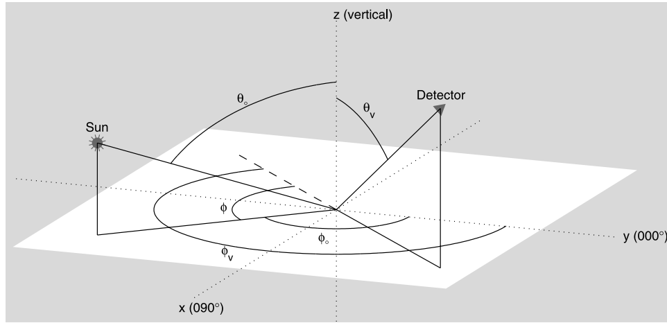
Figure 1. Definition of the solar zenith angle ( \theta_s ), the viewing zenith angle ( \theta_v ), the solar azimuth angle ( \phi_s ), the viewing azimuth angle ( \phi_v ), and the relative azimuth angle ( \phi ).
