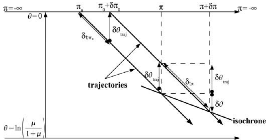
Fig. 1. Scheme for the derivation of the formula for isochrone slope.
