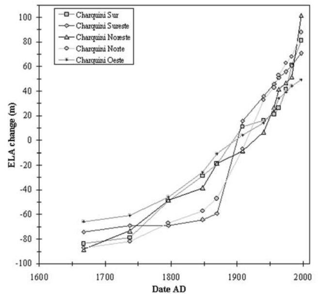
Fig. 4. Fluctuation of the ELA since the LIA maximum. The zero represents the average altitude of the ELA over the whole period.
