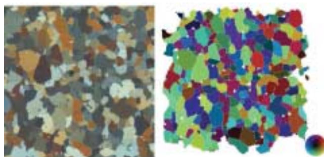
Fig. 1. Image of a thin section under cross-polarized light (left) and the corresponding texture (right). Grain boundaries appear white, and each grain defined within the microstructure has an orientation detailed in the colour map given by the polar plot projection shown on the bottom right.
