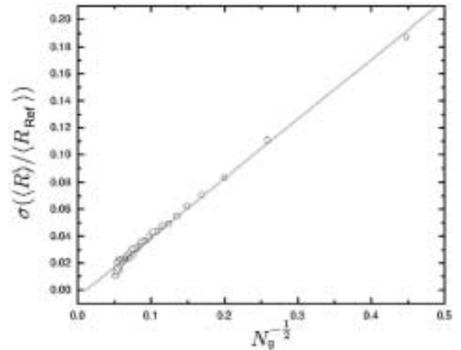
Fig. 3. Evolution of the standard deviation of \langle R \rangle over \langle R_{\text{Ref}} \rangle vs the inverse of the square root of the number of grains.
