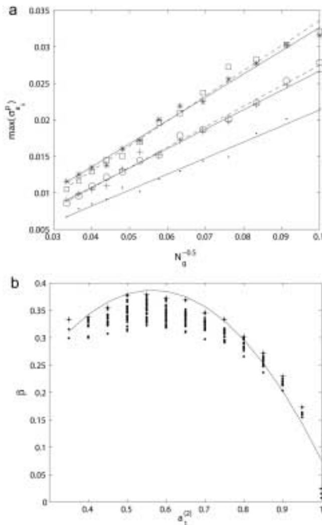
Fig. 6. (a) The \max(\sigma_{ii}^2) induced by the sampling of N_g grains over an initial population of 10 000. Dots: a_1^{(2)} = 0.9 , a_2^{(2)} = a_3^{(2)} = 0.05 ; crosses: a_1^{(2)} = 0.8 , a_2^{(2)} = 0.15 , a_3^{(2)} = 0.05 ; stars: a_1^{(2)} = 0.6 , a_2^{(2)} = 0.35 , a_3^{(2)} = 0.05 . The corresponding linear regressions are plotted as solid lines. Circles: a_1^{(2)} = 0.8 , a_2^{(2)} = 0.1 , a_3^{(2)} = 0.1 ; squares: a_1^{(2)} = 0.6 , a_2^{(2)} = 0.2 , a_3^{(2)} = 0.2 . The corresponding linear regressions are plotted as dashed lines. (b) Slope of the linear regression as presented in (a) vs (a_1^{(2)}) for the 231 textures tested. The maximum of each bin is marked with a cross, and corresponding second-order polynomial fit corresponds to the black curve.
