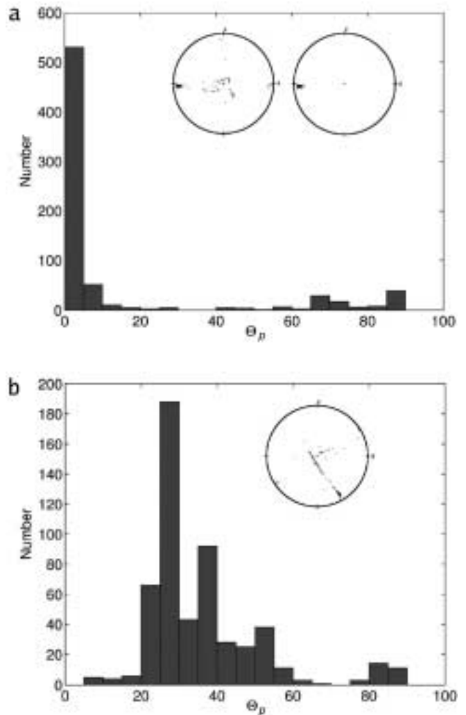
Fig. 5. (a) Distribution of the misorientation angle between ^\circ \mathbf{e}_1^k and all the pixels of grain k = 7 in the texture sampled at 1525.8 m on the EPICA Dome C ice core. The corresponding polar plot is also drawn (left). As this grain fulfils the condition for an included grain (see text), ^\circ \mathbf{e}_1^k is recalculated by excluding the pixels with a misorientation larger than 10^\circ . The corresponding polar plot is also plotted (right). (b) Distribution of the misorientation angle between ^\circ \mathbf{e}_1^k and all the pixels of grain k = 9 from the same thin section and the corresponding polar plot. This grain is rejected from the analysis.
