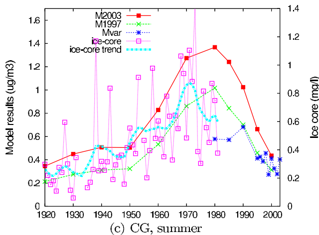
Figure 5. Comparison of modeled trends (model layer 13) and ice core records for sulfate at Col du Dôme (CDD) and Colle Gnifetti (CG). Dashed line with crosses is model simulations using 1997 meteorology (set 2), solid line with solid squares is model simulations using 2003 meteorology (set 3), dashed line with stars is model simulations using emissions and meteorology as appropriate for every year (set 4) dashed line with open squares is ice core record and thick dashed line is smoothed profile (first component of single spectra analysis with a 5-year time window). See section 4.4 for a description of the different sets. The ice core data have been inverted to air concentrations for CDD but not for CG.
