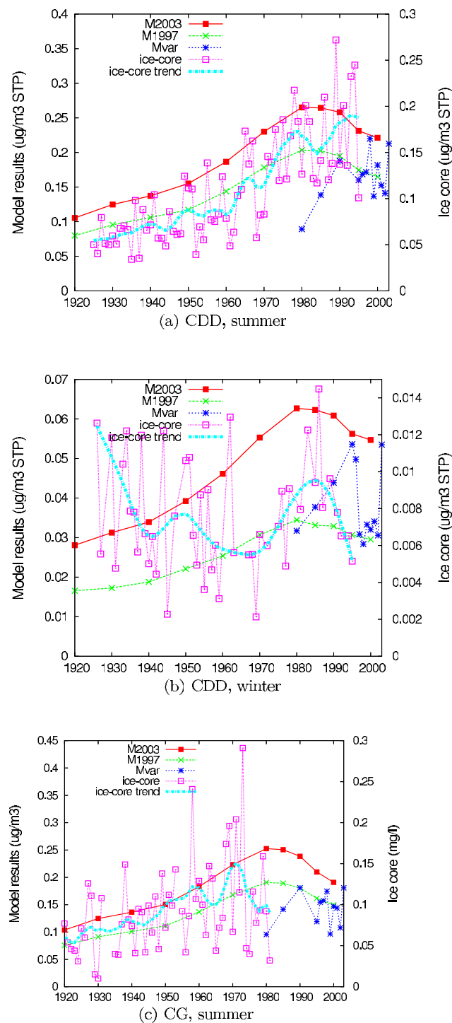
Figure 7. Comparison of modeled trends (model layer 13) and ice core records for NH x at Col du Dôme (CDD) and Colle Gnifetti (CG). Dashed line with crosses is model simulations using 1997 meteorology (set 2), solid line with solid squares is model simulations using 2003 meteorology (set 3), dashed line with stars is model simulations using emissions and meteorology as appropriate for every year (set 4), dashed line with open squares is ice core record and thick dashed line is smoothed profile (robust spline). See section 4.4 for a description of the different sets. The ice core data have been inverted to air concentrations for CDD but not for CG.
