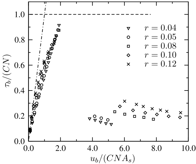
Figure 7. Friction law calculated for the ellipsoidal bedrock for different roughnesses ranging from r = 0.04 to r = 0.12 . C = 1.2 was adopted to plot all the curves. Same definition applies for dashed and dash-dotted lines as given in Figure 2.
