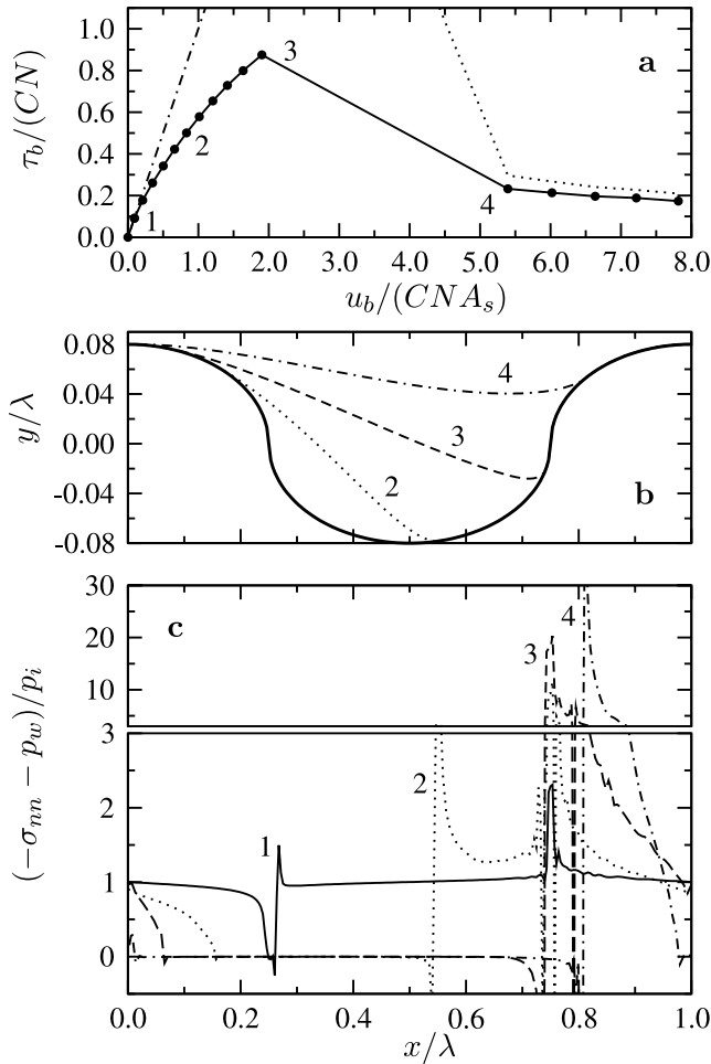
Figure 5. (a) Friction law calculated for the ellipsoidal bedrock of roughness r = 0.08 and a linear ice behavior (solid curve). The dotted curve represents the maximum positive bedrock slope restricted to the area of ice-bed contact, m_{\max}^{\text{contact}} , over C . The dash-dotted line corresponds to the friction law in the absence of cavitation. (b) Ellipsoidal bed and cavity shapes, and (c) normalized local effective pressure on the bed-cavity boundary for four different water-pressure levels labeled 1 to 4 in Figure 5a.
