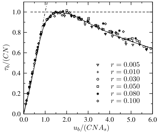
Figure 2. Friction law calculated for a sinusoidal bedrock and a linear ice rheology for different roughnesses ranging from r = 0.005 to r = 0.1 . C = 0.84 m_{\max} was adopted to plot all curves. Very good agreement is found with the semianalytical result of Schoof [2005] (solid curve). The dash-dotted line corresponds to the friction law in the absence of cavitation u_b = A_s \tau_b^n and the dashed line indicates the maximum value reached by \tau_b / (CN) .
