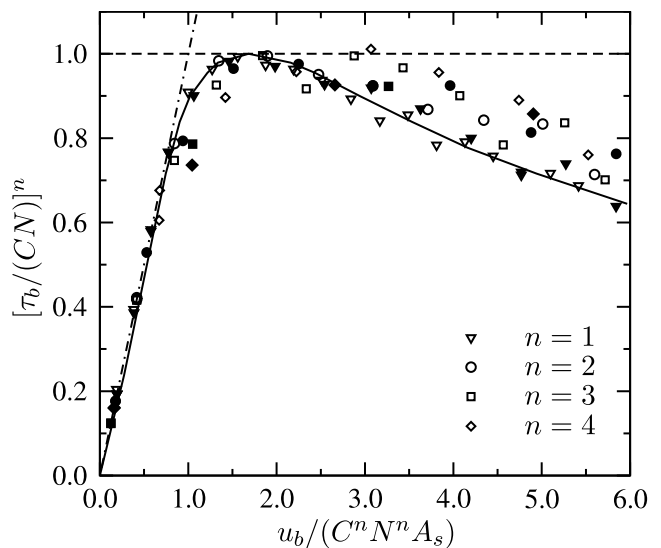
Figure 3. Friction law calculated for a sinusoidal bedrock for n = 1, 2, 3 and 4 for roughnesses r = 0.05 (open symbol) and r = 0.08 (solid symbol). C = 0.84 \pm 0.02 \times m_{\max} was adopted to plot all results. The solid line shows the semianalytical friction law obtained by Schoof [2005] in the case of a linear rheology. Same definition for dashed and dash-dotted lines as in Figure 2.
