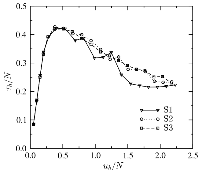
Figure 4. Influence of mesh refinement on the friction law for three different meshes defined in Table 2. Results are for a sinusoidal bedrock with r = 0.08 and n = 1 .
