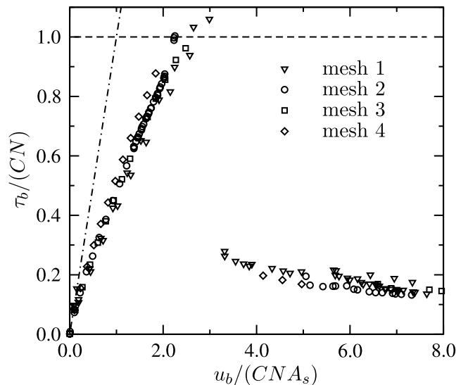
Figure 6. Friction law calculated for the ellipsoidal bedrock of roughness r = 0.05 for the four different meshes described in Table 3. C = 1.2 was adopted to plot all these curves. Same definition for dashed and dash-dotted lines as in Figure 2.
