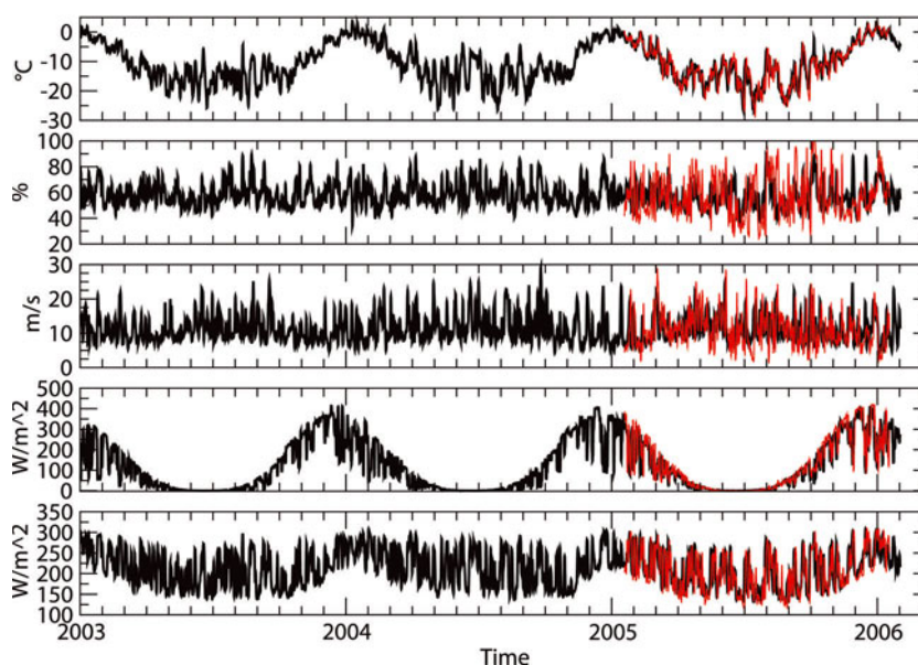
Fig. 7. Corrected ECMWF meteorology for Cap Prudhomme from 1 January 2003 to 31 January 2006 (black) and observed Cap Prudhomme meteorology (red): From top to bottom: temperature; relative humidity (with respect to liquid water); wind speed; downward solar and thermal radiation. All series smoothed with a 24 hour running filter.
