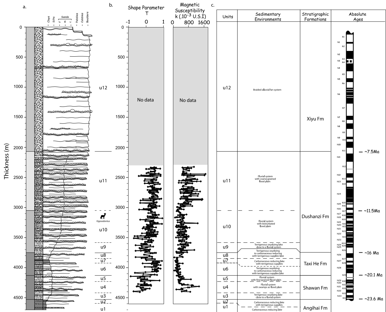
Figure 12. (a) Synthetic sedimentological column of the Jingou River section. (b) Depth evolution of shape parameter T and magnetic susceptibility k . (c) Comparison of the lithological units, stratigraphic formations and magnetostratigraphic ages.
