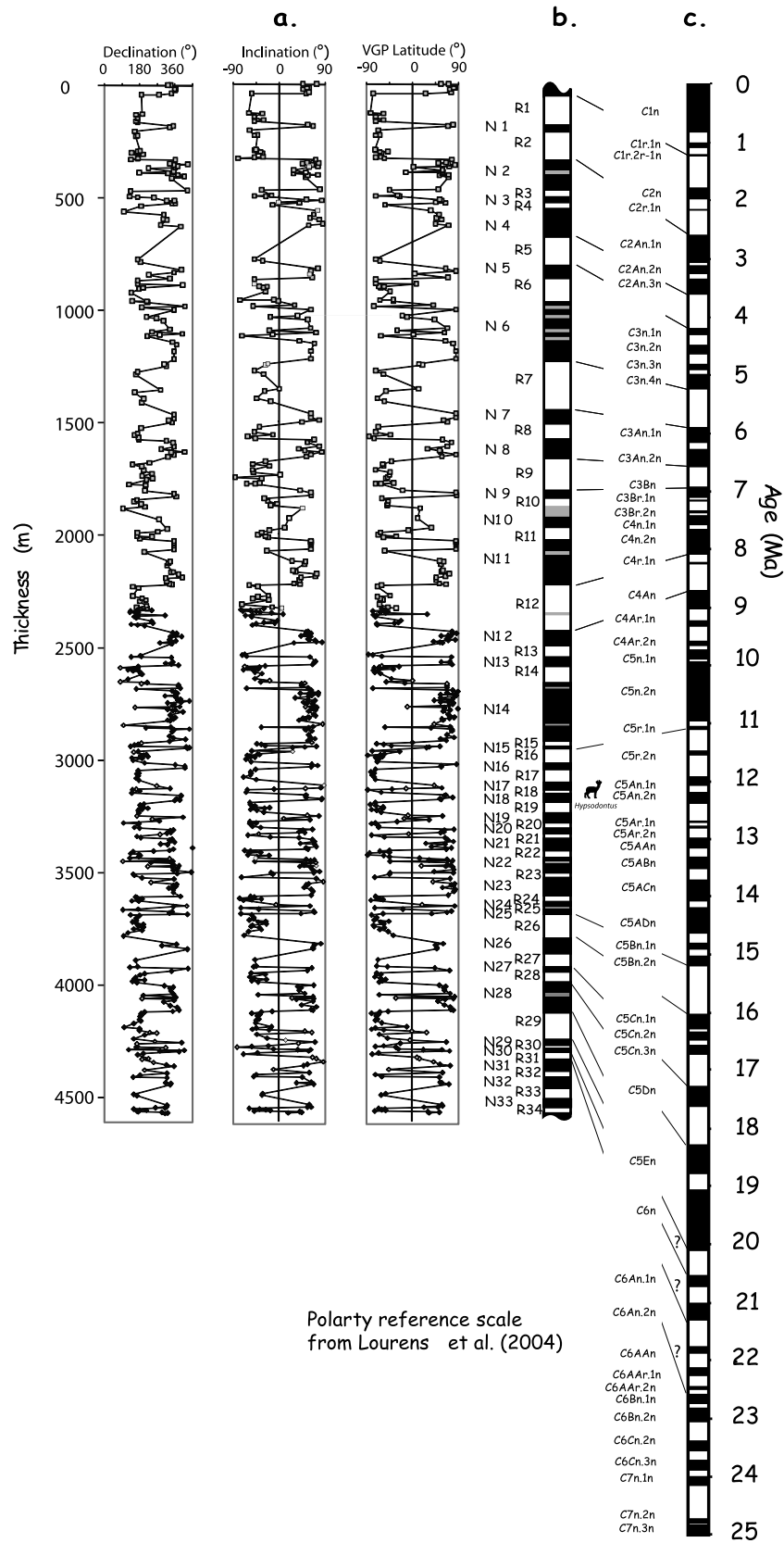
Figure 7. (a) Paleomagnetic directions (declination and inclination) obtained using principal component analysis. (b) Magnetostratigraphic column from this study. (c) Reference polarity timescale [after Lourens et al. , 2004].
