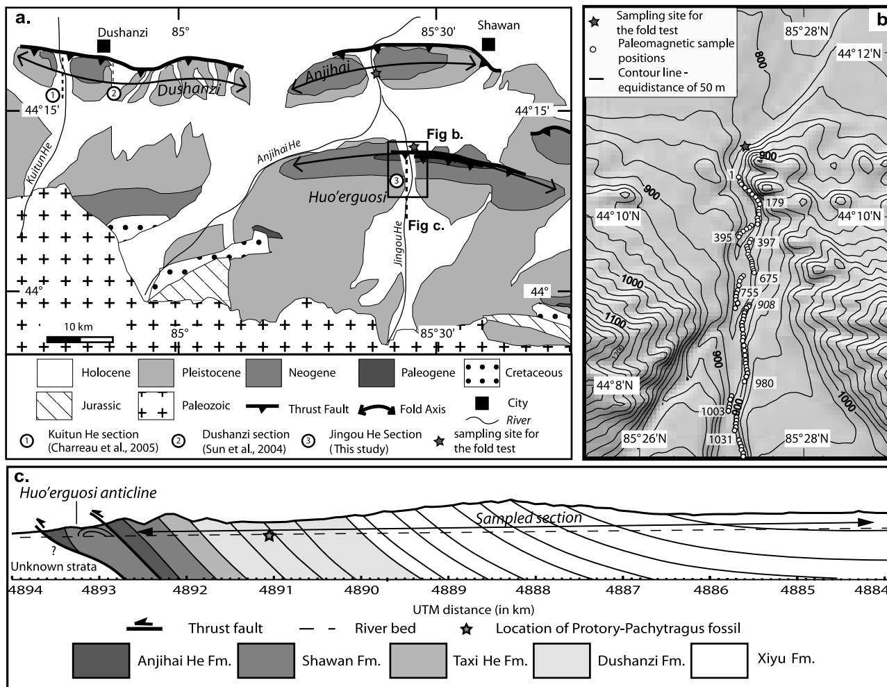
Figure 2. (a) Geological map of the Shawan area [after Avouac et al. , 1993] showing the location of the Kuitun section [ Charreau et al. , 2005], the Dushanzi section [ Sun et al. , 2004], and the Jingou River magnetostratigraphic section. (b) Detailed topographic map of the Jingou River section with sampling sites. (c) Cross section of the Huo'erguosi anticline indicating the location of the paleomagnetic cores and of Hypsodontus sp.
