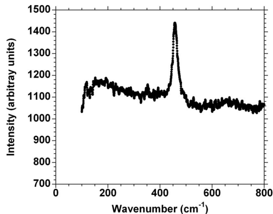
Fig. 2. Raman spectrum of the SiO 2 polymorph found in MM40. The ≈460 cm -1 line positively identifies it as quartz.
