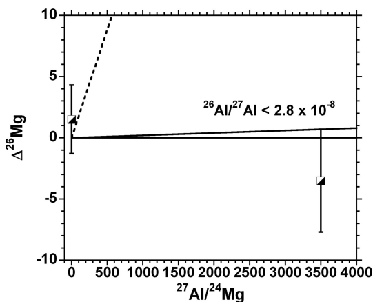
Fig. 6. Al-Mg isochron diagram for pyroxene (low Al/Mg ratio) and plagioclase (high Al/Mg ratio) in MM40. The ^{26}\text{Al}/^{27}\text{Al} = 4.5 \times 10^{-5} (dashed) and ^{26}\text{Al}/^{27}\text{Al} = 2.8 \times 10^{-8} (solid) lines are shown for reference.
