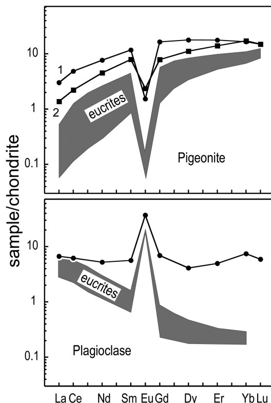
Fig. 5. CI normalized REE patterns for pyroxene and plagioclase from MM40. The shaded regions show the range of REE abundances observed in plagioclase and pigeonite from highly metamorphosed basaltic eucrites (28).
