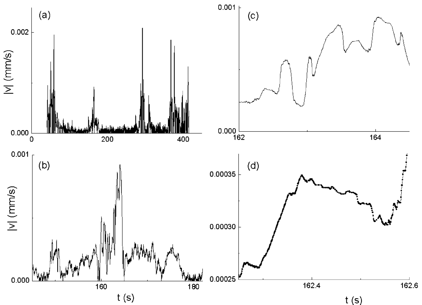
FIG. 4. Velocity signals from high-resolution extensometry derived from the displacement vs time record shown on Fig. 3. The long-term trend of the displacement-time curve on the time scale of the experiment was subtracted from the measured signal before derivation. Sequence of close-ups of the velocity signal shown in Fig. 5, suggesting scale invariance.
