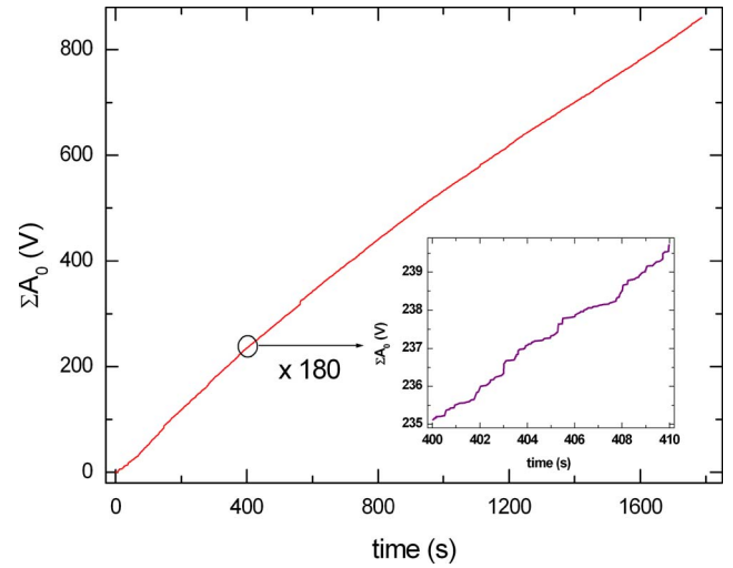
FIG. 7. (Color online) Compression creep experiment performed on an ice single crystals ( T = -10^\circ \text{C} ; and applied stress of 0.87 \text{ MPa} ). AE amplitudes cumulated from the onset of loading, \Sigma A_0 , as a function of creep time. \Sigma A_0 is a proxy of the total strain and its time evolution appears smooth at the scale of the entire test (main graph), although a staircaselike curve is observed when one focuses over a small time window (inset). This smoothing of the curve towards large time scales is the result of truncated distributions of dislocation avalanche sizes. This figure is very similar to the electromagnetic emission accompanying plastic deformation of ionic crystals that appears smooth at large time scale and staircase-like at small time scale (Ref. 33).
