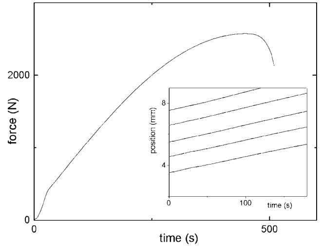
FIG. 3. Cu single crystal oriented for multislip loaded under uniaxial tension (thickness of 2 mm, width of 10 mm, length of 35 mm, Schmid's factor m=0.3 , and T=20^\circ\text{C} ). The applied strain rate is 5 \times 10^{-4} \text{ s}^{-1} . Macroscopic force vs time curve (main graph) and displacement vs time in five different locations along the sample (inset). The initial stage II hardening rate is \theta \approx 7E/1000 . The displacements were recorded at intervals of 1 mm in 20 sections of the samples.
