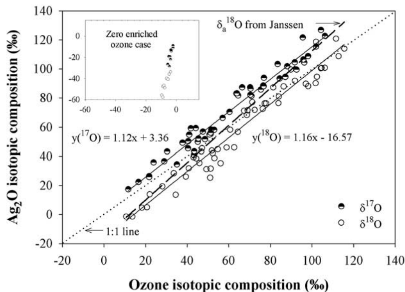
Figure 2. Correlation plot of \delta(\text{Ag}_2\text{O}) and \delta(\text{O}_3) showing that \delta values of silver-bound oxygen increase with increase in ozone \delta values in a linear fashion for both ^{17}\text{O} and ^{18}\text{O} . The \delta^{18}\text{O} values of \text{Ag}_2\text{O} are less than those of reacting \text{O}_3 because of chemical fractionation. In contrast, the \delta^{17}\text{O} values of \text{Ag}_2\text{O} are higher than those of \text{O}_3 because of fractionation and large position-dependent enrichment. The enrichment in terminal position (as calculated from the work by Janssen [2005]) is plotted to show the effect of fractionation. Samples with negligible enrichment (zero-enriched cases) have very different \delta values of \text{Ag}_2\text{O} as shown in inset.
