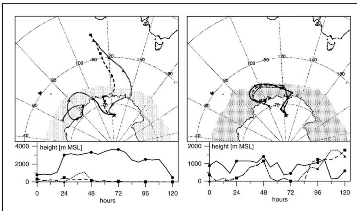
Figure 4. Example of 5 d backward trajectory in late July (left) and mid-September (right) when a moderate and strong sulfate depletion relative to sodium was observed on sea-salt aerosol at Concordia, respectively. Grey areas refer to the sea-ice cover. Dotted marks indicate the location every day. The plot are combined to corresponding monthly mean satellite derived sea ice map [Comiso, 1990, updated 2007] available on the Web at http://nsidc.org/ .
