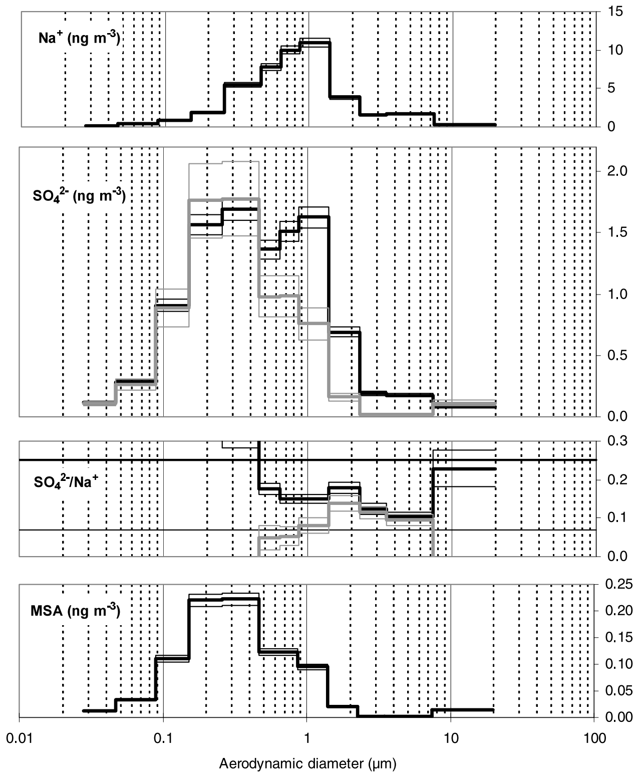
Figure 3. Mass size distribution of \text{Na}^+ , \text{SO}_4^{2-} , and MSA of the aerosol sampled at Concordia 9 to 23 September. Also plotted is the \text{SO}_4^{2-}/\text{Na}^+ ratio calculated for the larger particles. For \text{SO}_4^{2-} levels and the \text{SO}_4^{2-}/\text{Na}^+ ratio, the grey curves refer respectively to the biogenic fraction of sulfate estimated from MSA (see section 4), and to the ratio R' (see text) corrected from this biogenic fraction.
