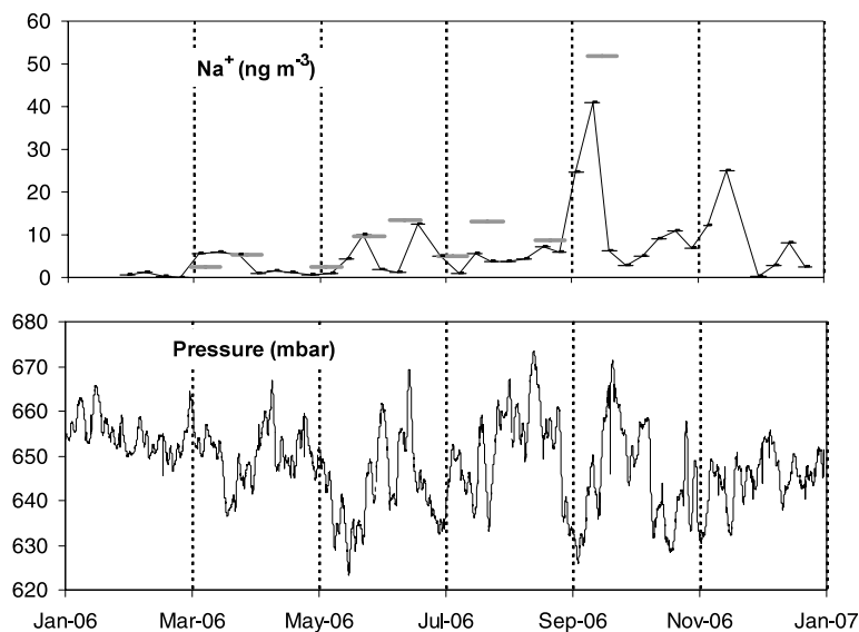
Figure 1. (top) 2006 year-round record of sodium from bulk filters (in black) and of the sum of concentrations observed on the 12 stages of the impactor (in grey). (bottom) Local atmospheric pressure at Concordia. Horizontal bars reported on the sodium curves refer to the sampling time interval. Pressure data are from the Concordia Automatic Weather Station (AWS 8989) of University of Wisconsin-Madison (available on the ftp address: ftp://amrc.ssec.wisc.edu/pub/aws/ ).
