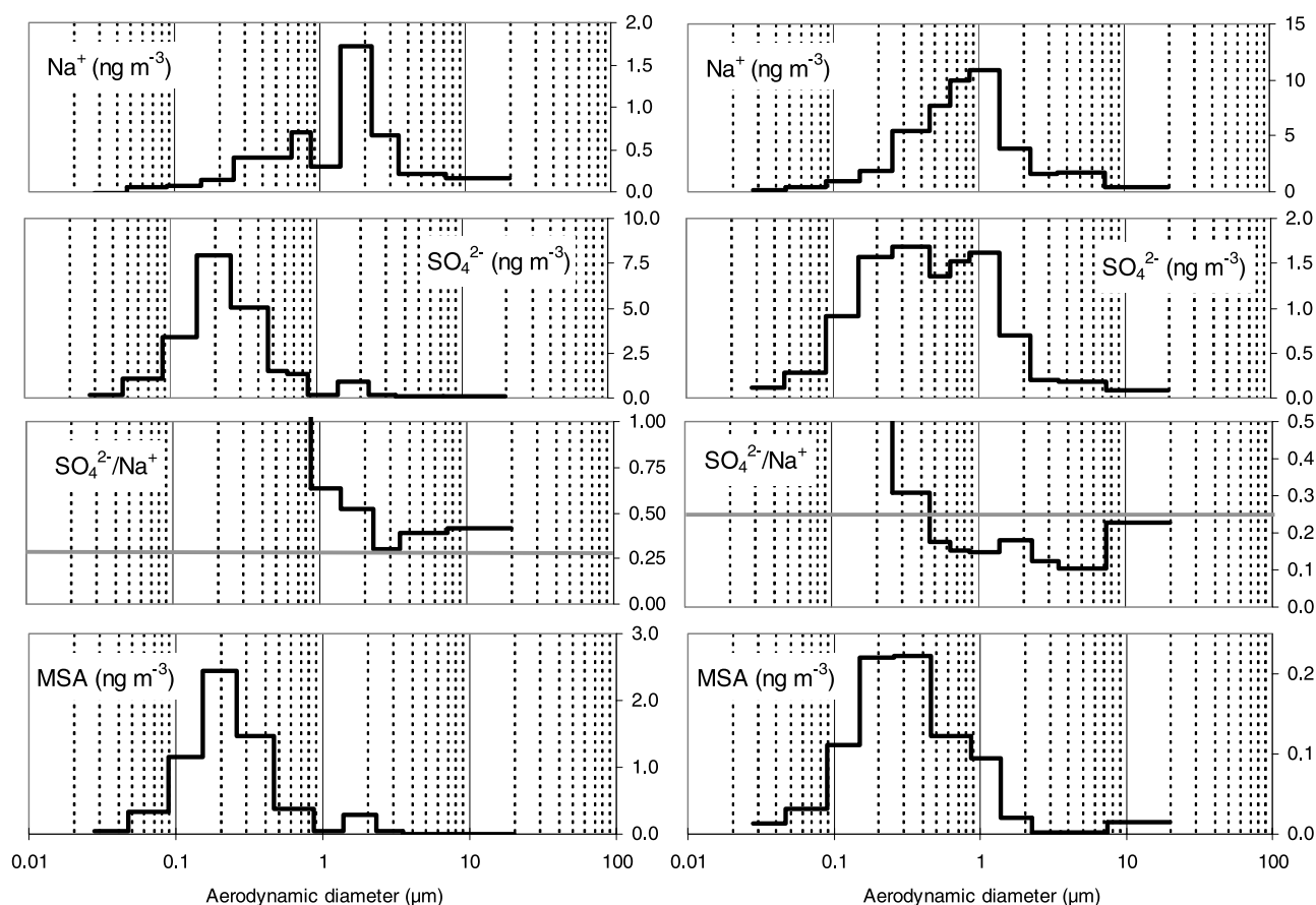
Figure 2. Mass size distribution of \text{Na}^+ , \text{SO}_4^{2-} , and MSA of aerosol sampled at Concordia between 21 March and 4 April 2006 (left) and 9 to 23 September (right). Also reported is the \text{SO}_4^{2-}/\text{Na}^+ ratio calculated for the larger particles.
