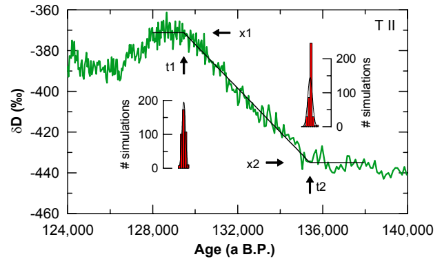
Fig. 2. Example of RAMPFIT results for \delta\text{D} at Termination II. The black line represents the ramp that best fits the data based on weighted least-squares regression. Arrows indicate the levels x_1 and x_2 and the change points t_1 and t_2 . The histograms show the change points for 400 bootstrap simulations. The distribution of these simulated change points is used to derive an estimate of the uncertainty of the change points.
