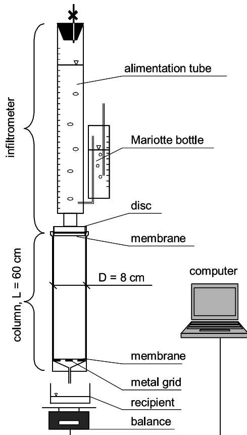
Figure 1. Experimental setup.
