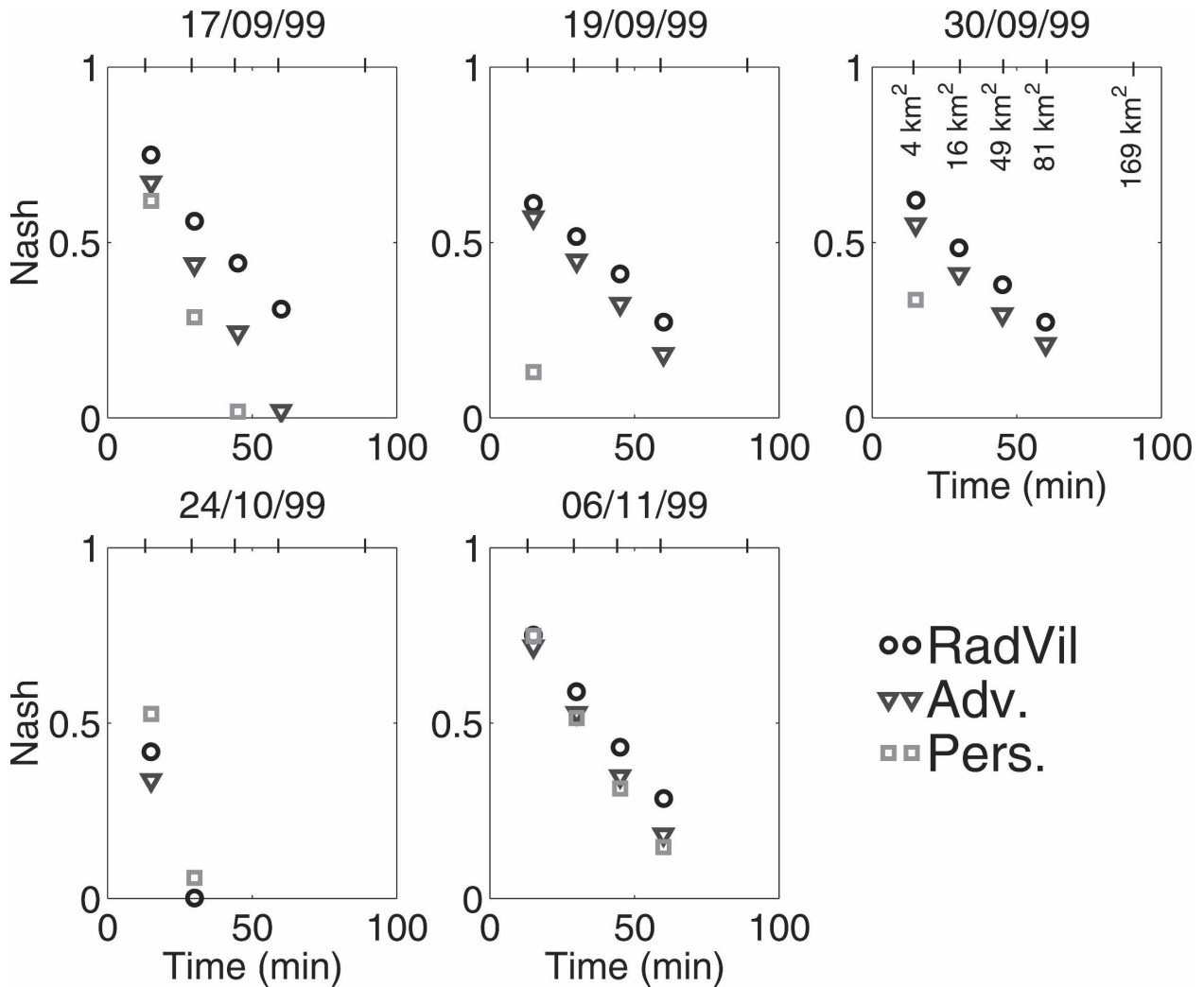
FIG. 5. Quantitative evaluation of RadVil on the five case studies: Nash criterion as function of catchment response time (corresponding to a surface area, indicated on the rhs) for cumulated rainfall by the three rainfall forecasting methods.
