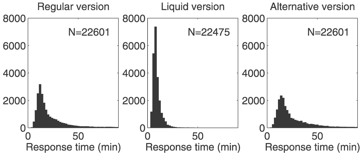
FIG. 6. Response time as function of the VIL estimate technique for the first case study (17 Sep 1999).
