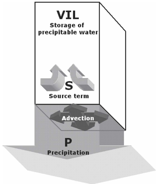
FIG. 1. Schematic representation of RadVil.
