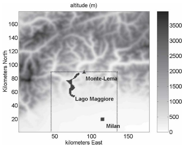
FIG. 2. Topography of area target. RadVil is performed and tested in the area delimited by the dashed box.
