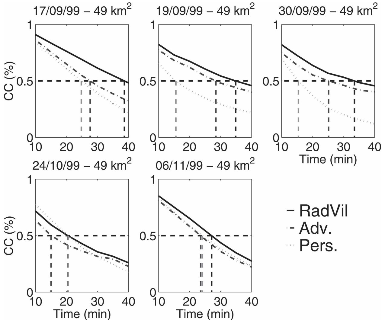
FIG. 4. Quantitative evaluation of RadVil on the five case studies: correlation coefficient as function of forecast time for cumulated rainfall on 49 km 2 catchments by the three rainfall forecasting methods. The limits of predictability of the three methods are represented by the vertical dashed lines.
