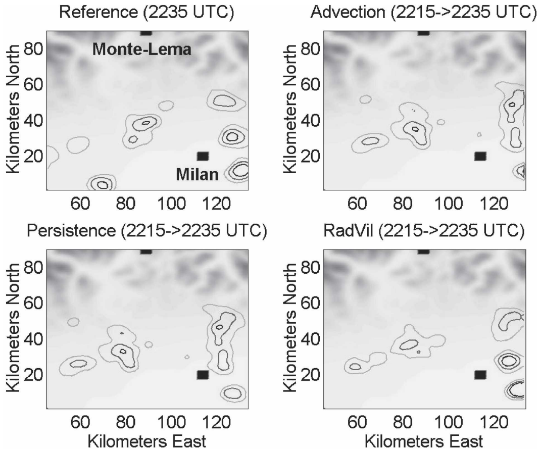
FIG. 3. Qualitative evaluation of RadVil on the first case study (17 Sep 1999): x - y plot of the (top left) reference rainfall at 2235 UTC, and (bottom left) the forecast of the persistence model (equal to the reference field at 2215 UTC), (top right) the advection model, and (bottom right) RadVil for 2215 UTC + 20 min. The x and y axes are given in km. The rainfall isohyets are contoured with spacings of 10, 20, 30, and 40 \text{mm h}^{-1} .
