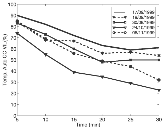
FIG. 7. RTAC Coefficient of VIL fields on the five case studies.
