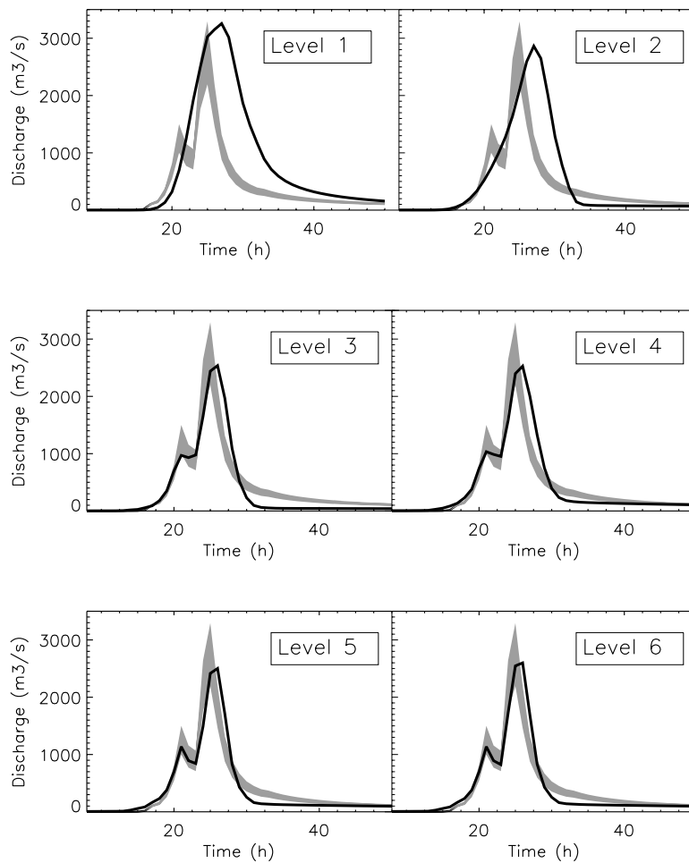
Figure 3. Discharge simulations at the Anduze station (Gardons river, 545 km 2 ), for the 6 levels of spatial information. Observed discharges are figured in grey (with indicative 20% uncertainty intervals). Simulated discharges are figured in black.
