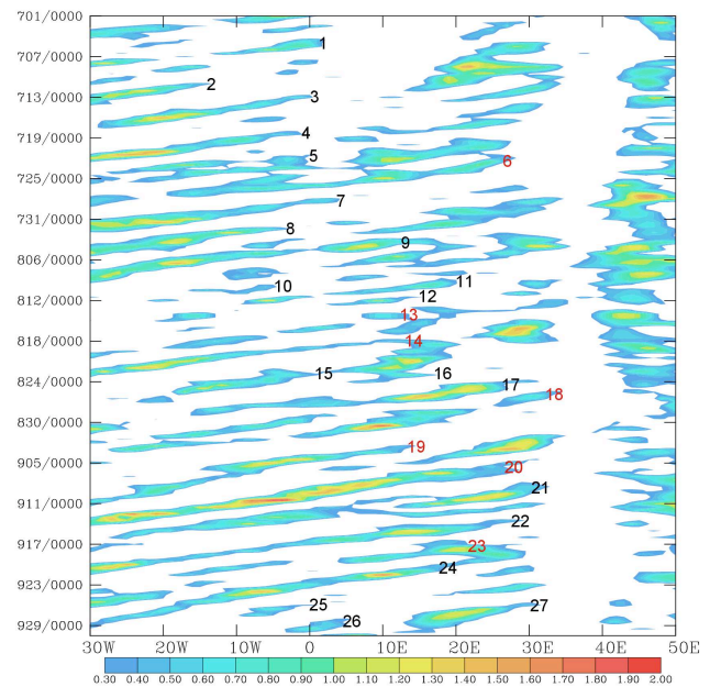
Fig. 19. Hovmoeller space-time diagram of 700 hPa curvature vorticity averaged between 5^{\circ}\text{N} and 15^{\circ}\text{N} based on NCEP analysis. The numbers refer to synoptic systems that meet the tracking criterion used by Berry et al. (2007). Those in red became tropical cyclones in the Atlantic basin. These were Chris (6), Ernesto (13), Debby (14), Florence (18), Gordon (19), Helene (20), Isaac (23). On the vertical axis time is expressed as month-day/hour.
