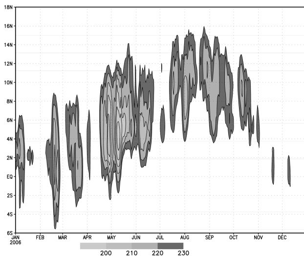
Fig. 6. Time-latitude cross-section of the OLR field averaged on 10° W–10° E in 2006. A moving average on \pm 3 days have been applied to smooth the signal. The coastline is located approximately at 5° N. Only values lower than 230 \text{ W m}^{-2} are shaded.
