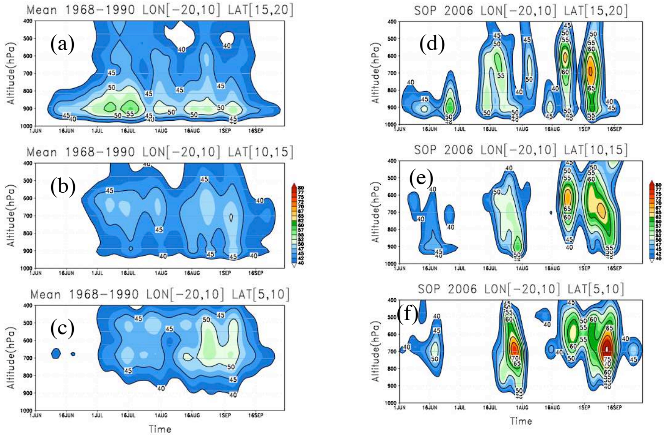
Fig. 18. Vertical and spatial distribution of the mean AEW activity, using wavelet analysis of the daily meridional wind, over the West Africa and near Tropical Atlantic in 3 domains; longitudes 20^{\circ} W– 10^{\circ} E, latitudes 15^{\circ} N– 20^{\circ} N, 10^{\circ} N– 15^{\circ} N and 5^{\circ} N– 10^{\circ} N. Left panels (a, b, c) show the 1968–1990 climatology, right panels (d, e, f) the AMMA summer SOP.
