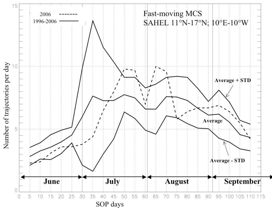
Fig. 8. Five-day average of C3+C4 MCS tracks numbers per day detected over the Sahelian area 11^{\circ}\text{N} – 17^{\circ}\text{N} / 10^{\circ}\text{W} – 10^{\circ}\text{E} including a 10-day running average (see details in the text). The black lines represent the evolution of the mean 1996–2006 track numbers as well as the evolution for the mean plus and minus one standard deviation, and the dashed line the 2006 evolution. The x-axis labels are expressed in days from 1 June.
