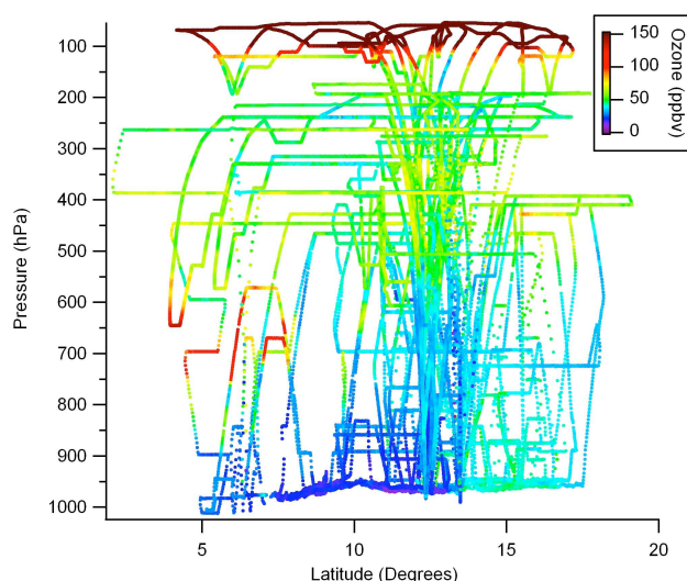
Fig. 28. Flight tracks for the BAe-146, the DLR Falcon, the French Falcon and the M55 between 20 July and 21 August plotted as a function of latitude and altitude and coloured by the ozone concentration. Note that the ozone concentrations above 100 hPa are off the colour scale, extending up to 1700 ppb.
