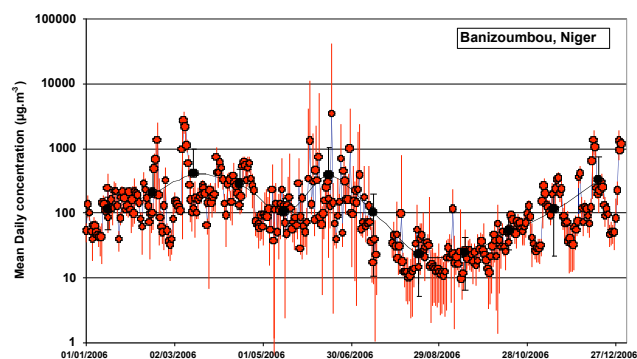
Fig. 27. Daily mean atmospheric concentrations of particulate matter lower than 10\text{ }\mu\text{m} ( \text{PM}_{10} ) (red dots) and daily standard deviations (red bars) measured in Banizoumbou (Niger, 13.31^\circ\text{ N}/2.66^\circ\text{ E} ; see its location on Fig. 1) in 2006. The black dots represent the monthly means and standard deviations (note that the daily mean concentrations have been computed based on a selection of raw data using wind direction criterions to select only dust transport wind sectors).
