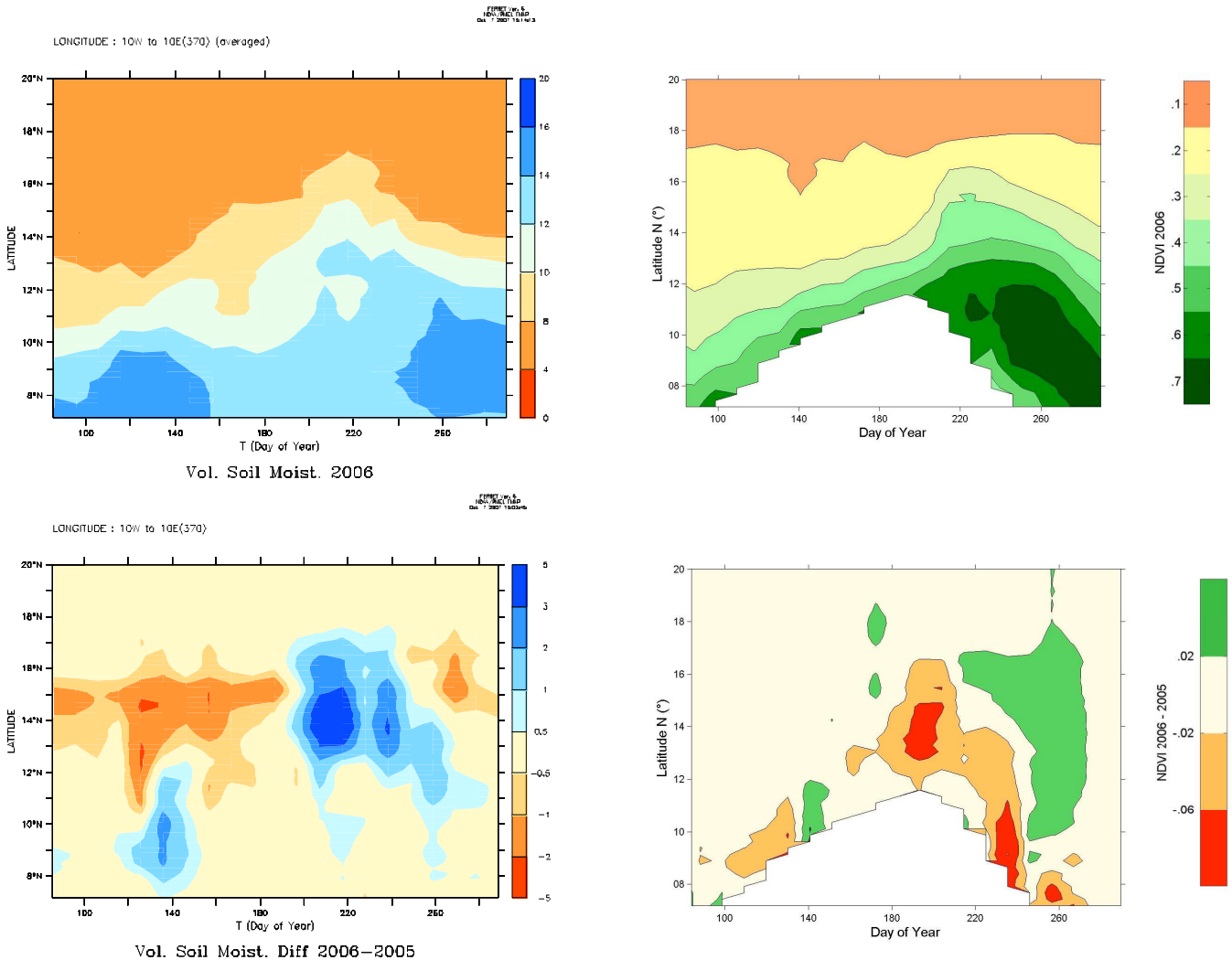
Fig. 24. Time-latitude diagram of 2006 (top) and 2006–2005 anomaly (bottom) of (left) surface soil moisture ( \% \text{ m}^3 \text{ m}^{-3} ) and (right) NDVI, averaged between 10^\circ \text{ W} and 10^\circ \text{ E} . Regions of persistent cloud contamination are shown in white on the NDVI plot. The x-axis labels are expressed in days from 1 January.
