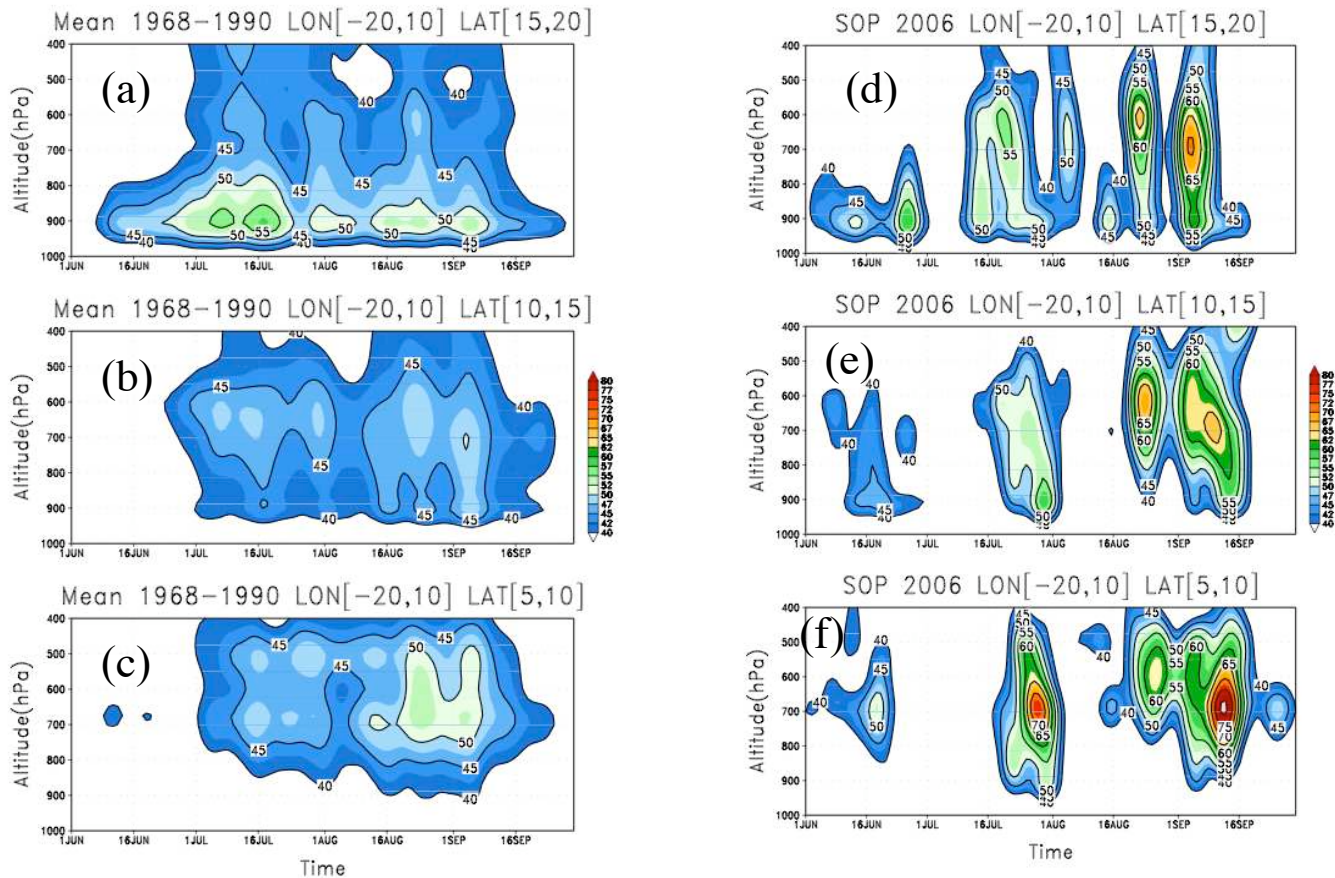
Fig. 18. Vertical and spatial distribution of the mean AEW activity, using wavelet analysis of the daily meridional wind, over the West Africa and near Tropical Atlantic in 3 domains; longitudes 20^{\circ} W– 10^{\circ} E, latitudes 15^{\circ} N– 20^{\circ} N, 10^{\circ} N– 15^{\circ} N and 5^{\circ} N– 10^{\circ} N. Left panels (a, b, c) show the 1968–1990 climatology, right panels (d, e, f) the AMMA summer SOP.
