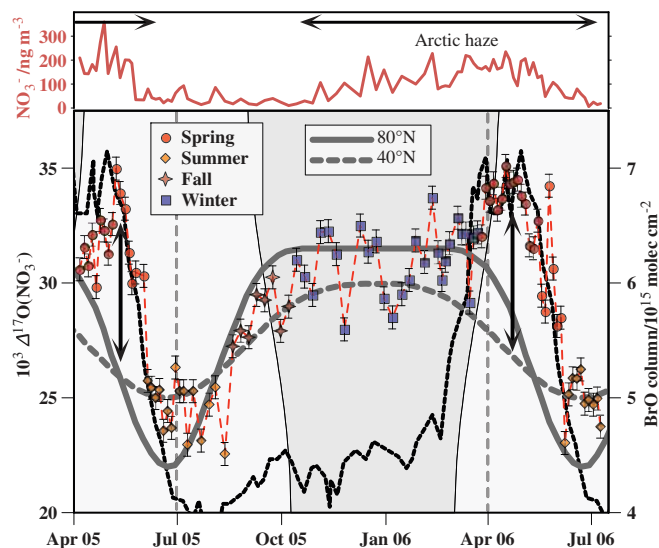
Fig. 1. Seasonal cycle of concentrations and \Delta^{17}\text{O} of atmospheric nitrate at Alert. Also shown is the day length (from 0 to 24 hours, the shaded area corresponding to nighttime conditions). The black dashed line represents a satellite-retrieved column of BrO north of 70°N (32). Thick gray lines correspond to the calculated \Delta^{17}\text{O} value in atmospheric nitrate formed at 40° and 80°N, respectively. The black vertical arrows indicate the strong deviation from these seasonal cycles in spring, due to the interaction of BrO with snowpack-emitted \text{NO}_x . The vertical dotted lines are identical to those in Fig. 2 (delineating periods of snowpack \text{NO}_x emissions from April to June).
